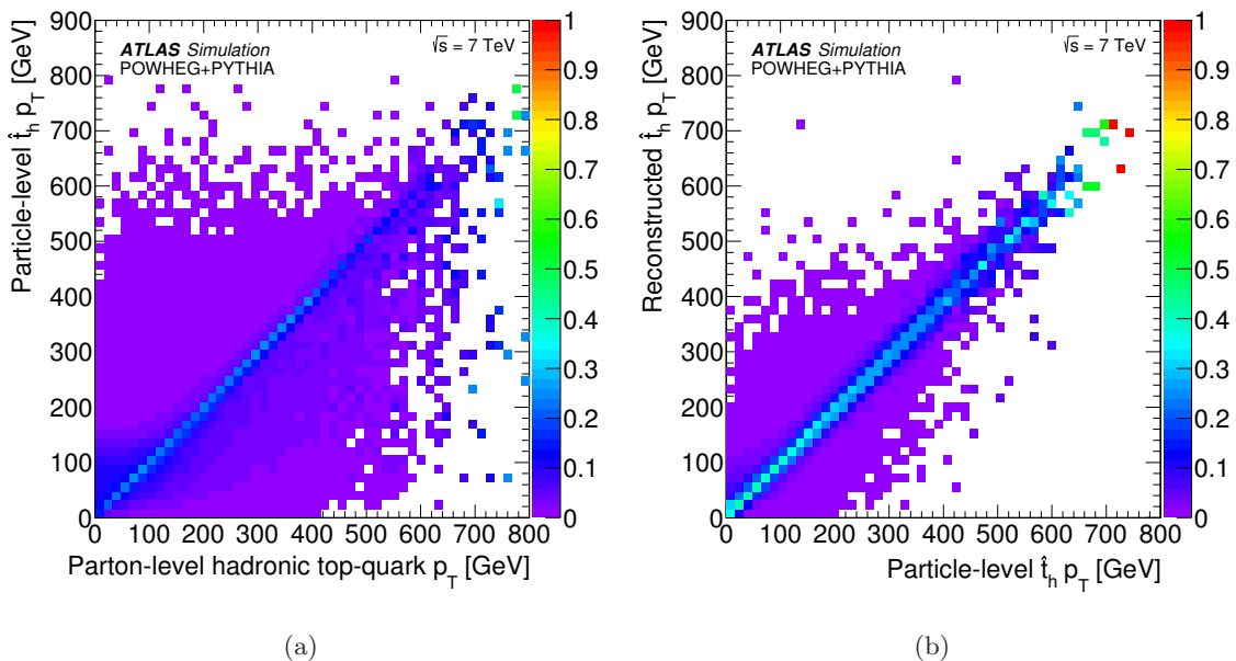
Figure 2. (a) Monte Carlo study using the nominal POWHEG+PYTHIA MC sample showing the correlation between the parton-level top-quark p_T and the particle-level hadronic pseudo-top-quark p_T . (b) Monte Carlo study showing the correlation between the particle-level hadronic pseudo-top-quark p_T and the hadronic pseudo-top-quark p_T evaluated from reconstructed objects. In each case the correlation is normalised to all the events within a bin on the horizontal axis.
