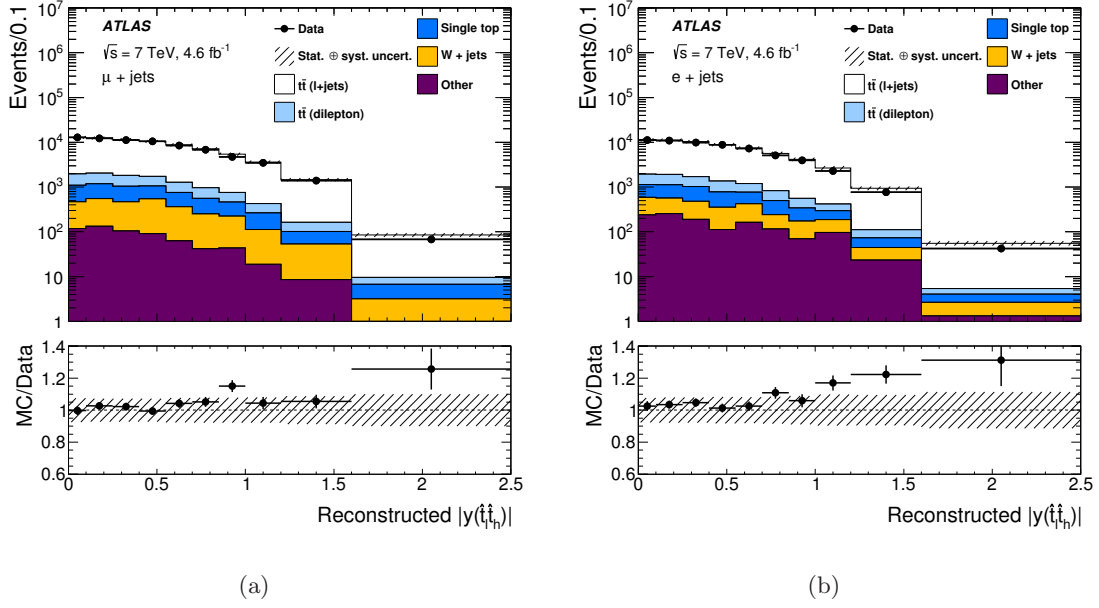
Figure 6. The reconstructed rapidity for the pseudo-top-quark system \hat{t}_1 \hat{t}_h in comparison to the MC signal and data-driven background models. The y(\hat{t}_1 \hat{t}_h) distributions: (a) the muon channel and (b) the electron channel. Signal and background processes are shown in different colours, with “Other” including small backgrounds from diboson and Z + \text{jets} production, as well as non-prompt and fake leptons from multi-jet processes. The POWHEG+PYTHIA MC generator with the Perugia 2011C tune is used for the t\bar{t} signal estimate. The shaded band shows the total systematic and statistical uncertainties on the signal plus background expectation.
