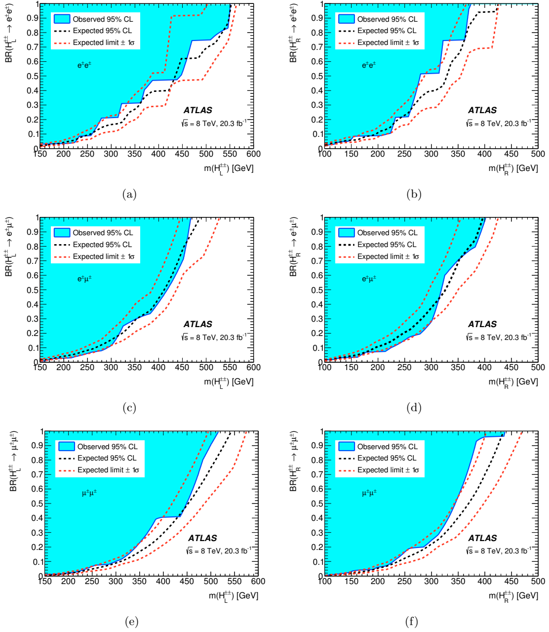
Figure 5: Observed and expected 95% CL limits on H_L^{\pm\pm} \rightarrow \ell^\pm \ell^\pm (left column) and H_R^{\pm\pm} \rightarrow \ell^\pm \ell^\pm production (right column) in the branching ratio versus H^{\pm\pm} mass plane for the e^\pm e^\pm (top), e^\pm \mu^\pm (middle) and \mu^\pm \mu^\pm (bottom) channel. The blue shaded area is excluded.
