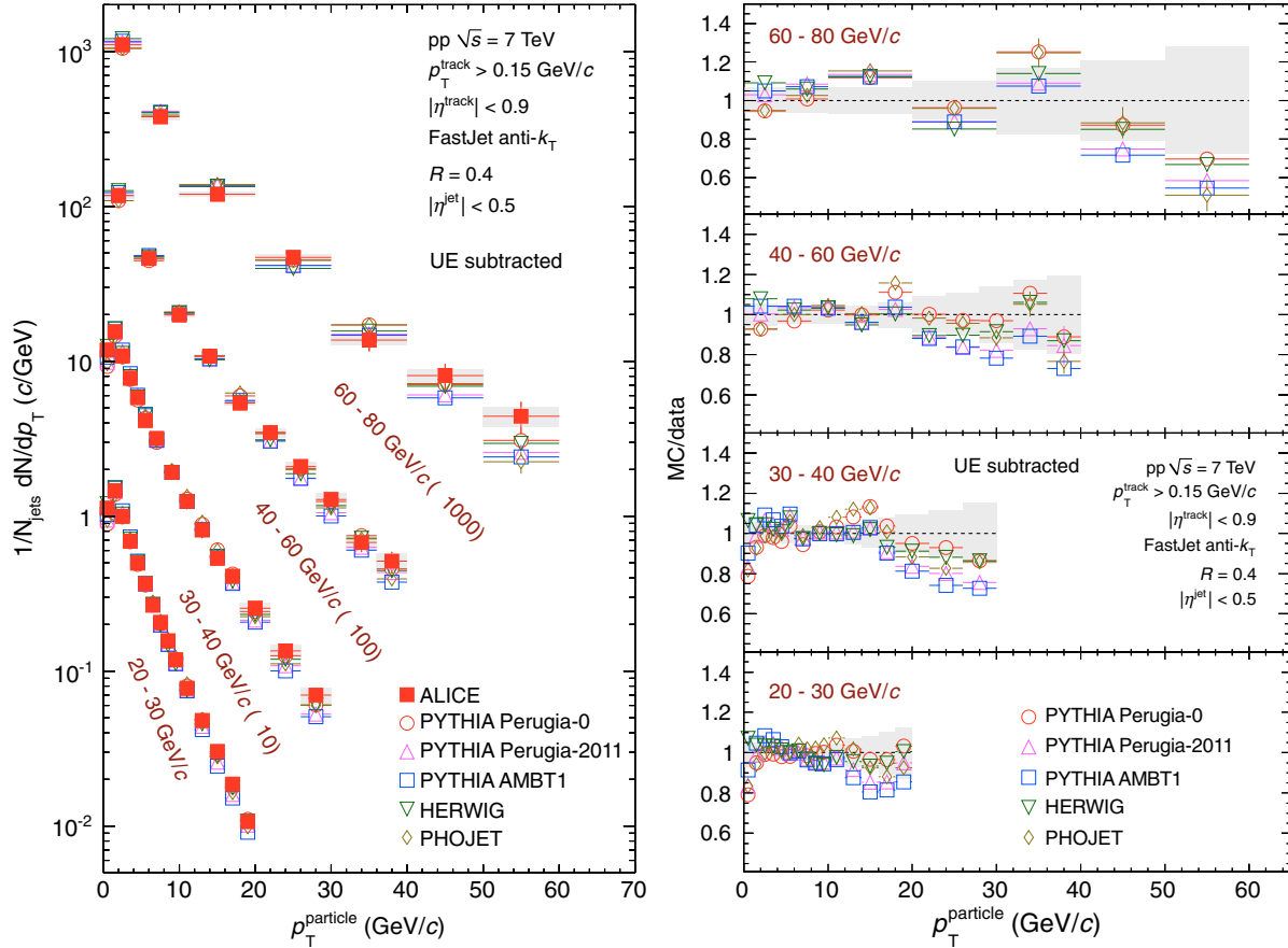
FIG. 12 (color online). Left panel: Charged particle p_T spectra dN/dp_T in leading jets for different bins in jet transverse momentum, compared to simulations. For simulations, the UE contribution is subtracted. Right panel: Ratio of simulations to data. The shaded band indicates the quadratic sum of statistical and systematic uncertainties on the data.
