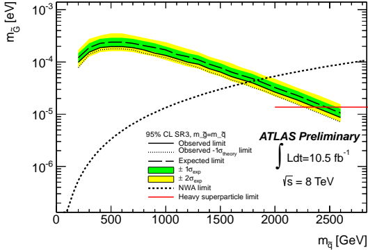
Figure 4: Observed and expected 95% CL lower limits on the gravitino mass as a function of the squark mass for degenerate squark/gluino masses. The solid red line denotes the current limit from LEP [30] on the gravitino mass assuming very heavy squarks/gluino.
