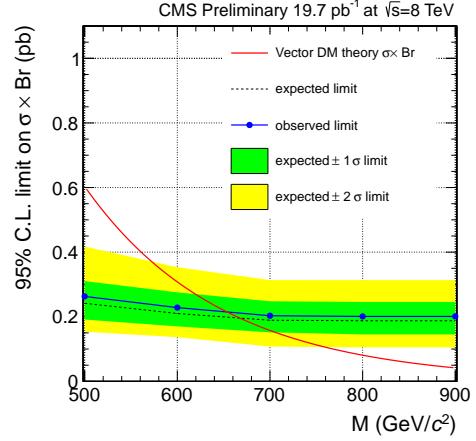
Figure 7: The 95% CL expected and observed CL_s limits as a functions of the mass of the DM candidate for the vector DM model. The theory cross section is also shown with a red solid line.
