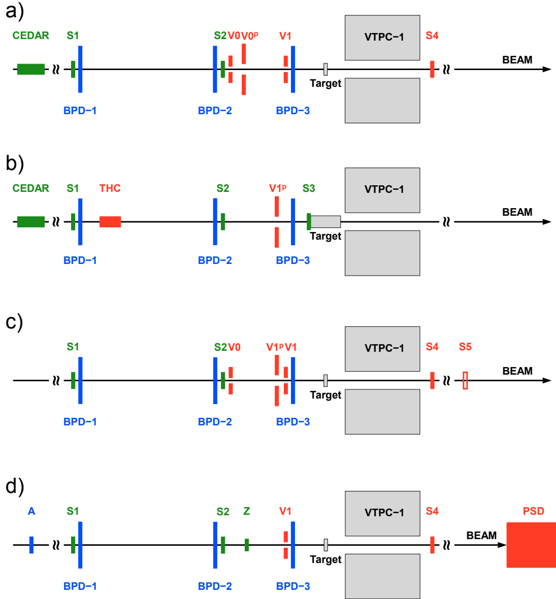
Figure 8. Schematic layout (horizontal cut in the beam plane, not to scale) of the beam detectors in four configurations of the beamline, see text for details.
