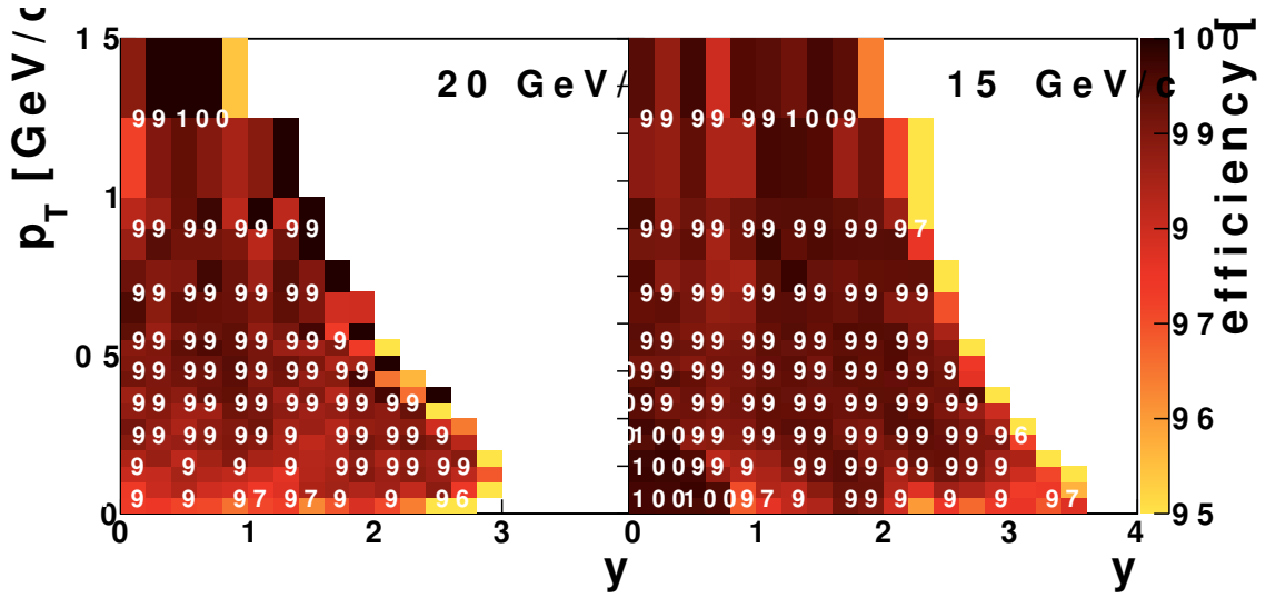
Figure 18. The reconstruction efficiency of negatively charged pions produced in p+p interactions at 20 ( left ) and 158 GeV/c ( right ) as a function of pion rapidity and transverse momentum. The magnetic fields were set for a total bending power of 1.1 and 9 Tm at 20 and 158 GeV/c, respectively.
