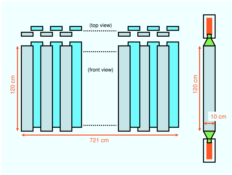
Figure 23. The schematic layout of scintillators in the ToF-F detector.
