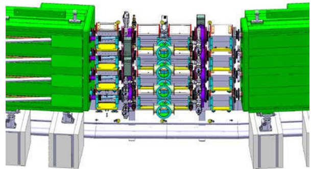
Figure 3: Injection period modified for injection of 160 MeV H^- ions from Linac4. In-between two main dipole magnets there is a system of 4 chicane dipoles, with the stripping foil unit in its center. Every ring is equipped with its proper injection hardware.
