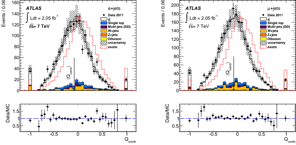
Figure 7. Distribution of the combined charge, Q_{\text{comb}} , in electron+jets (left) and muon+jets (right) final states. The full circles with error bars are data, the full black line corresponds to the SM scenario, and the dashed red line corresponds to the exotic model. The vertical line, labeled with \langle Q_{\text{comb}} \rangle , shows the mean value of the Q_{\text{comb}} distribution obtained from data. Only statistical uncertainties are shown.
