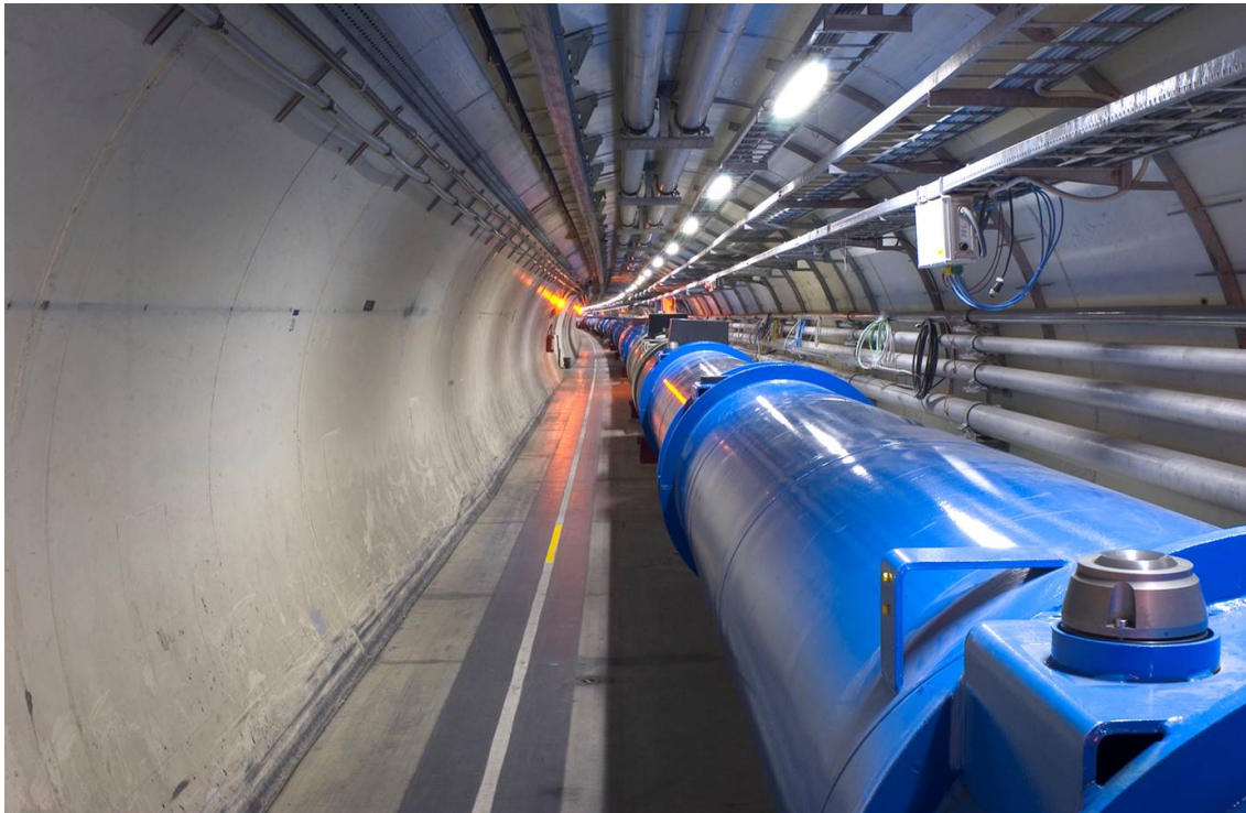
Figure 1.1: Photograph of a section of the LHC already installed in the tunnel.
