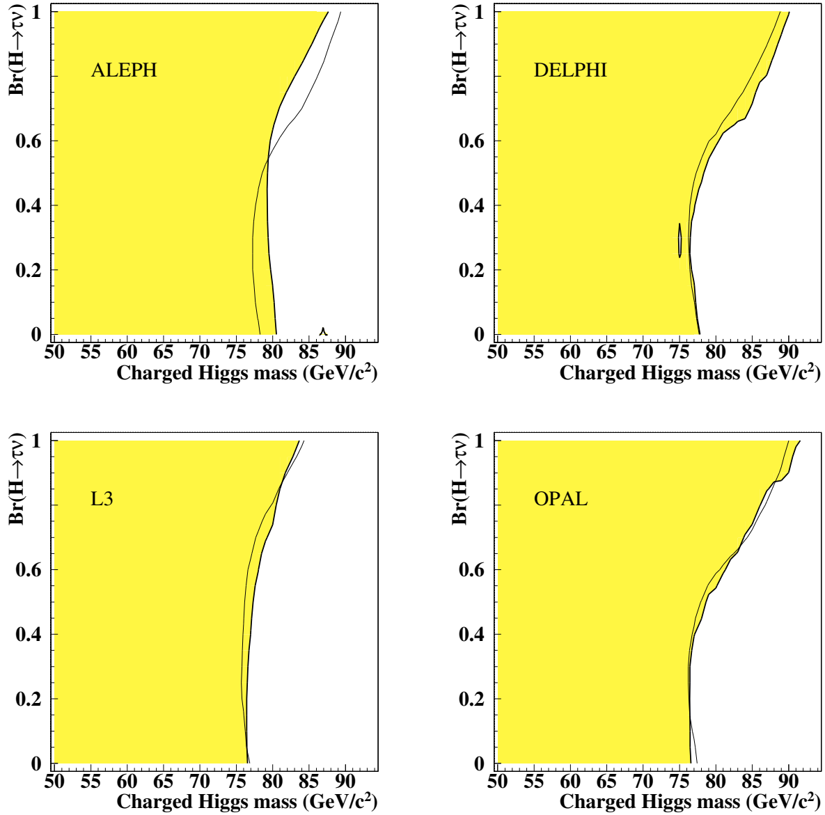
Figure 1: Type II 2HDM: the 95% C.L. bounds on m_{\text{H}^\pm} as a function of the branching ratio \text{Br}(\text{H}^+ \rightarrow \tau^+ \nu) , for each of the four LEP experiments separately. The expected exclusion limits are indicated by the thin solid line and the observed limits by the thick solid line. The shaded area is excluded at the 95% C.L. or higher.
