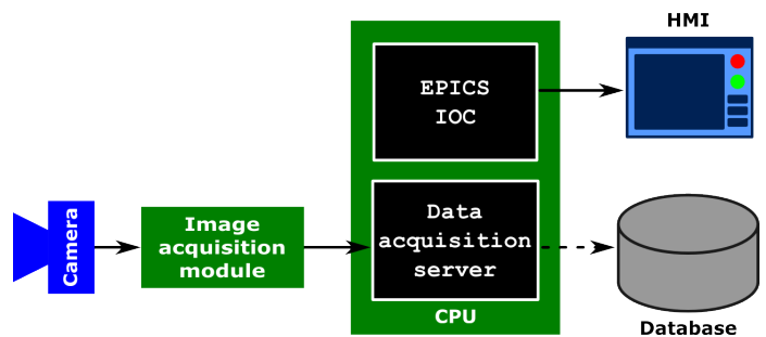
Fig. 5. Structure of image acquisition system
