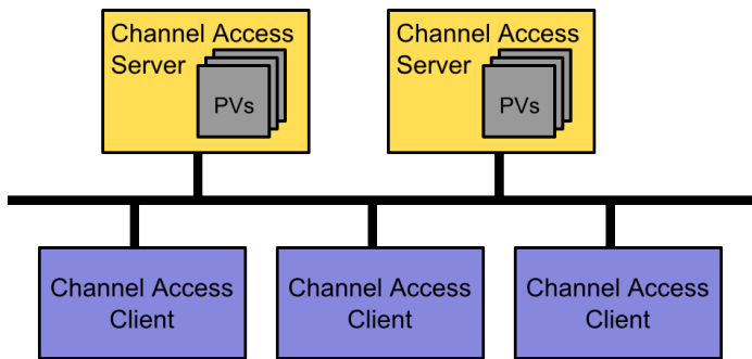
Fig. 2. EPICS architecture
