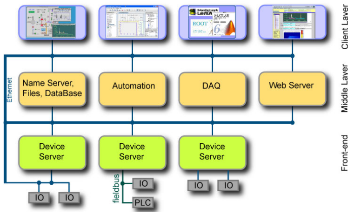
Fig. 1. The DOOCS architecture overview
