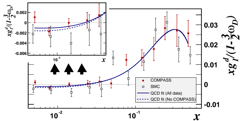
Figure 2.4: Values of xg_1^d(x) measured by COMPASS (full circles) and SMC (open squares) for Q^2 > 1 \text{ (GeV/c)}^2 . The curves represent the results of the fits at the Q^2 of the COMPASS points (solid line for all data, dashed line with COMPASS excluded). The data points are corrected for the deuteron D-wave state probability \omega_D = 0.05 (i.e. they correspond to the published values of g_1^d divided by 0.925).
