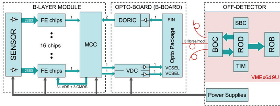
Fig. 1. Block scheme of the ATLAS Pixel Detector DAQ system from the front-end chip FE-I3 to the readout modules where full events are built and pushed to the higher trigger levels (ROB).
