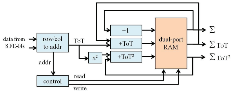
Fig. 4. Histogramming unit as implemented in the data path FPGA. Occupancy, ToT and (\text{ToT})^2 histograms are produced requiring minimal resources. Data are stored in a dual-port memory and sent later to the external PC farm to for fits and extraction of the calibration constants.
