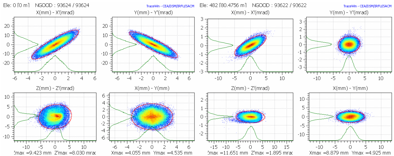
Figure 4.13. D^+ phase space at the linac input (left) and output. 99% emittance ellipse in red.
