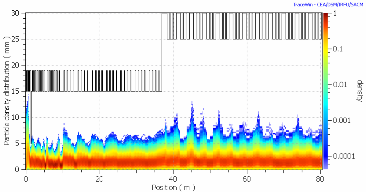
Fig 4.14. Particle density distribution along the linac for D^+ .
