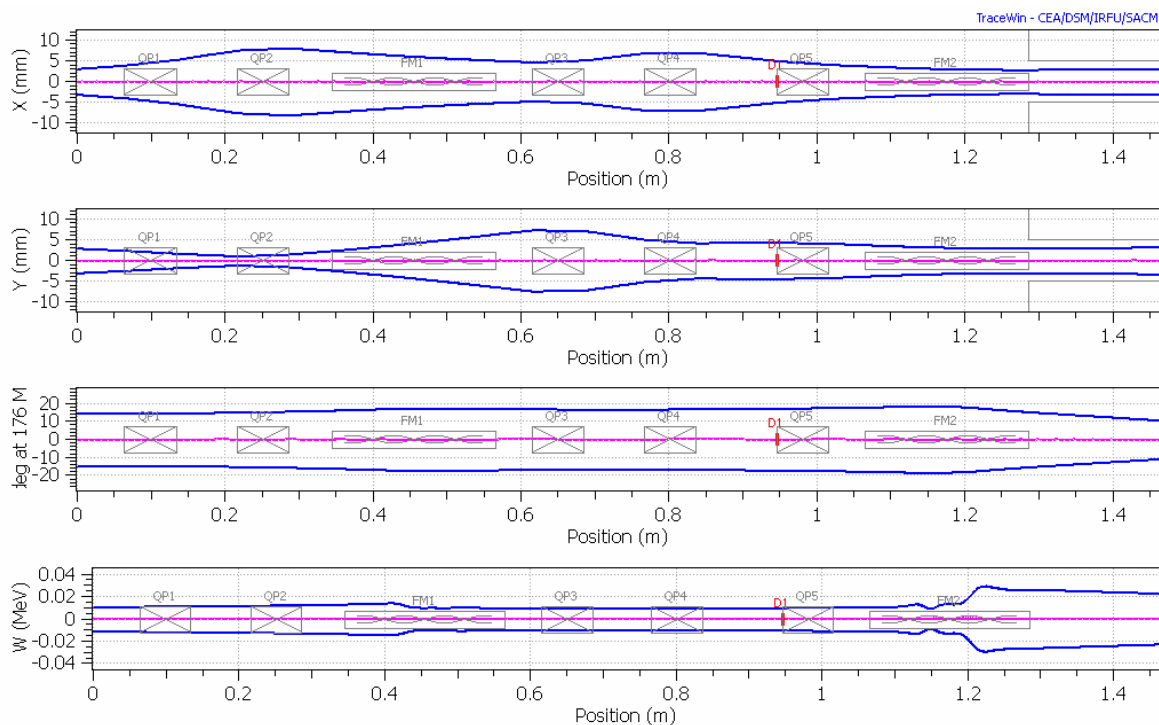
Fig. 4.3. H - Beam envelope in the MEBT.
