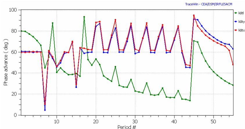
Fig. 4.1. Phase advance per period vs. period number for the H beam.
