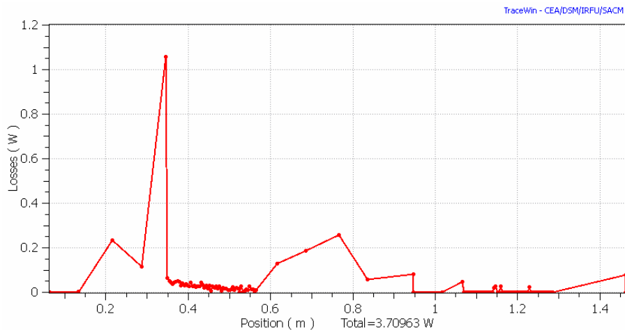
Fig. 4.7 Beam power loss distribution along the MEFT for H - beam, caused by the particles transmitted, but not accelerated, in the RFQ.
