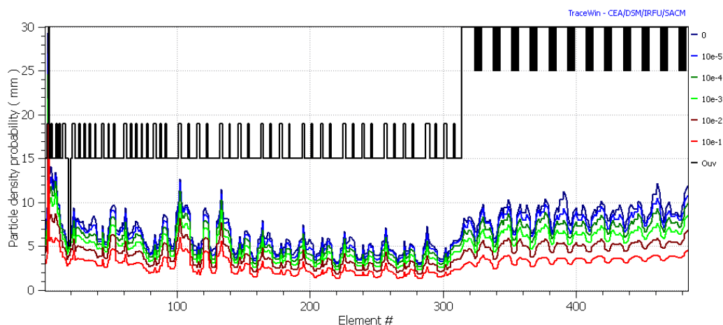
Fig. 4.6. H + particle density probability along the Low- and Medium- \beta linac, simulated with 500000 macroparticles. Sum of 100 runs of 5000 macro particles with different sets of random errors.
