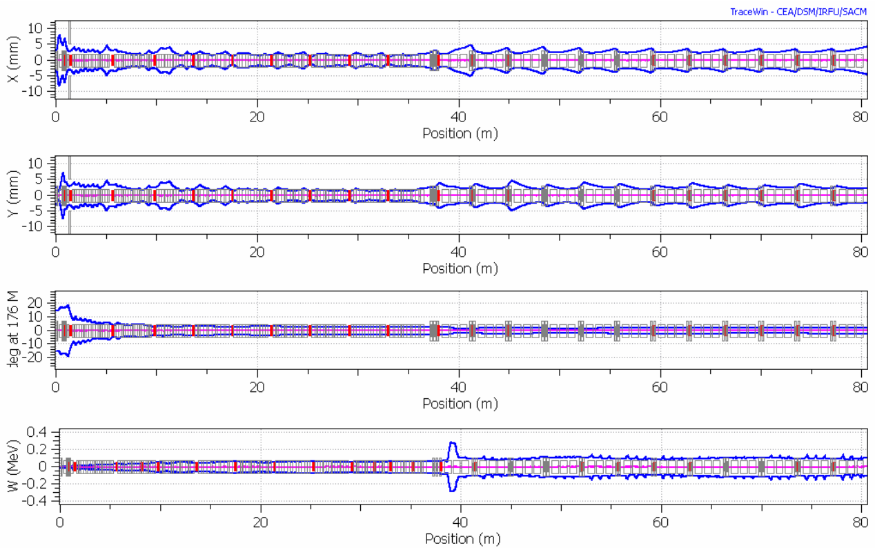
Fig. 4.8. 2 rms envelope plot for H^- .
