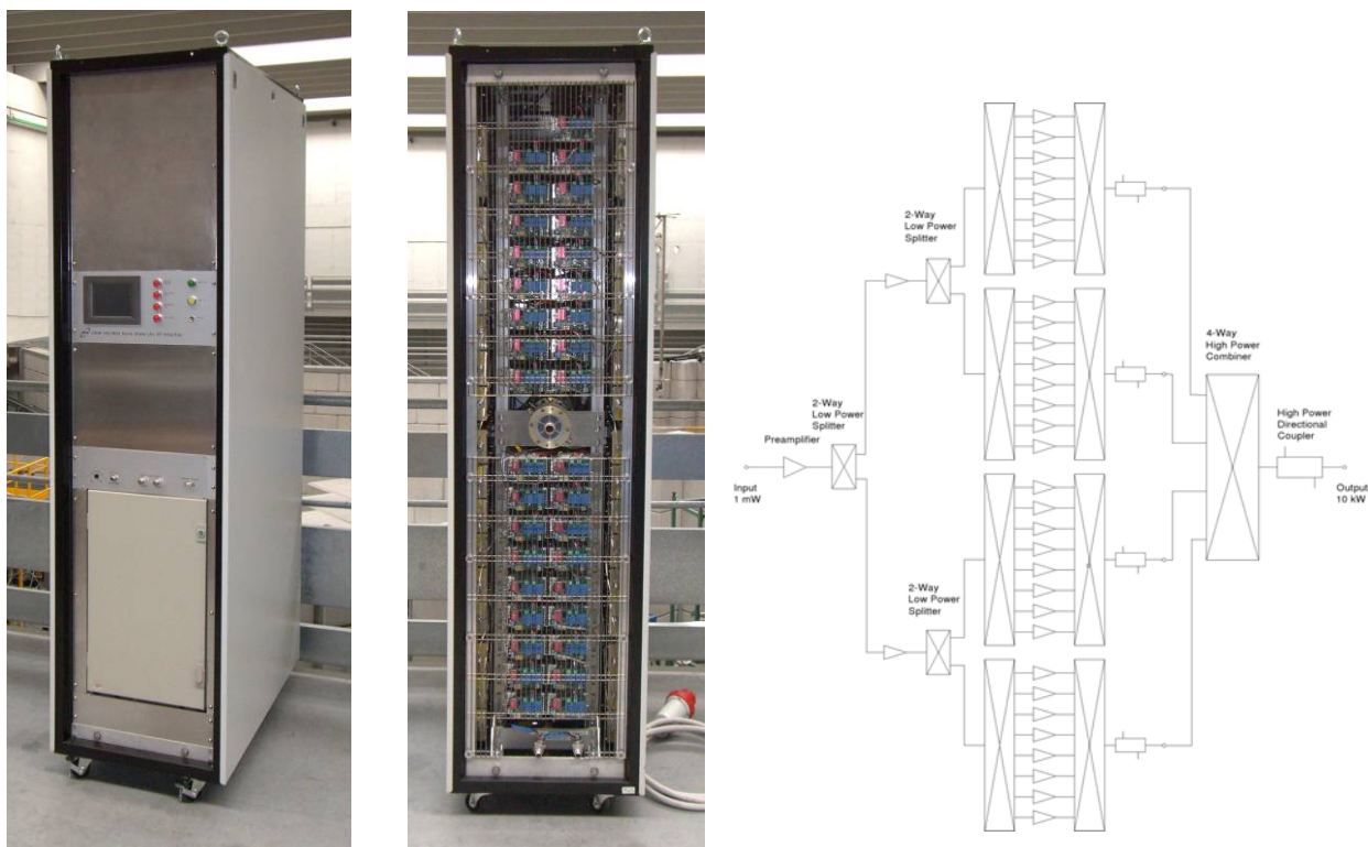
Fig. 5.13 Left: The EURISOL 10 kW amplifier, front and rear views. Right: the rf amplifier block diagram.
