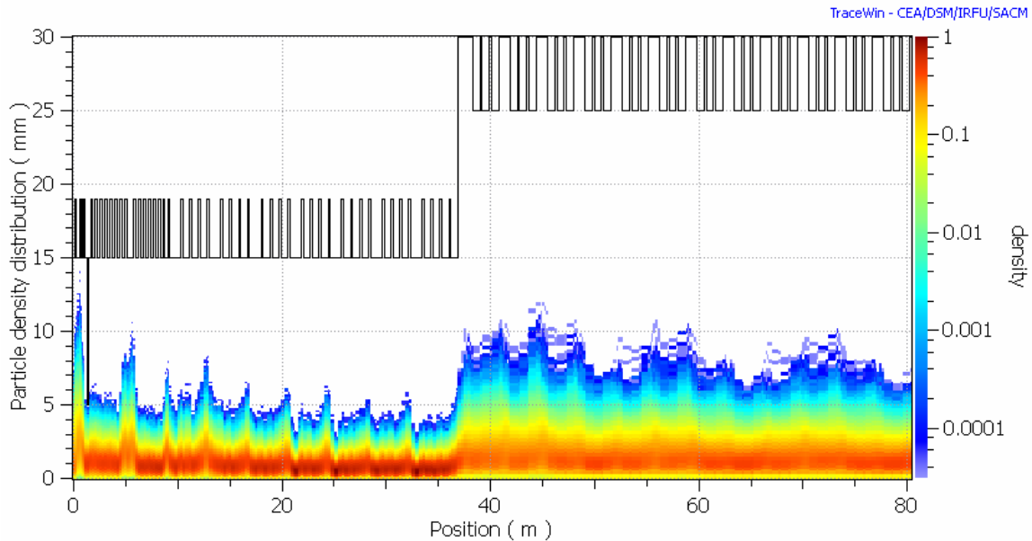
Fig 4.18. Particle density distribution along the linac for ^3\text{He}^{++} .
