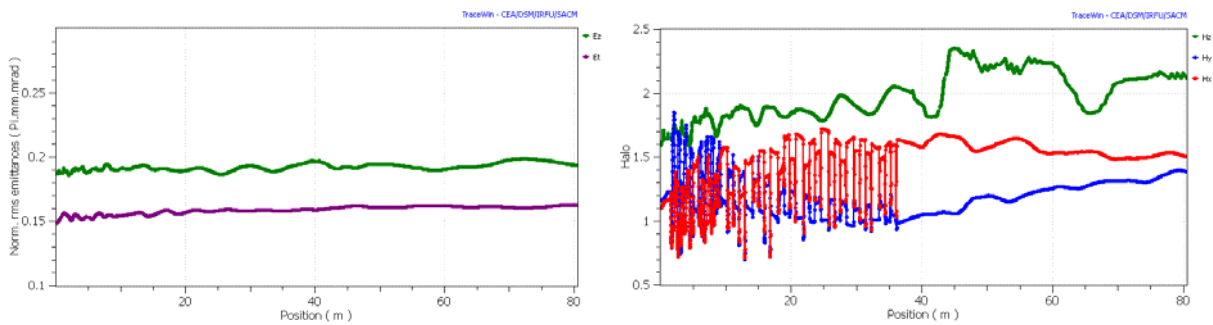
Figure 4.15. Emittance evolution (left) and halo parameter along the linac for D^+
