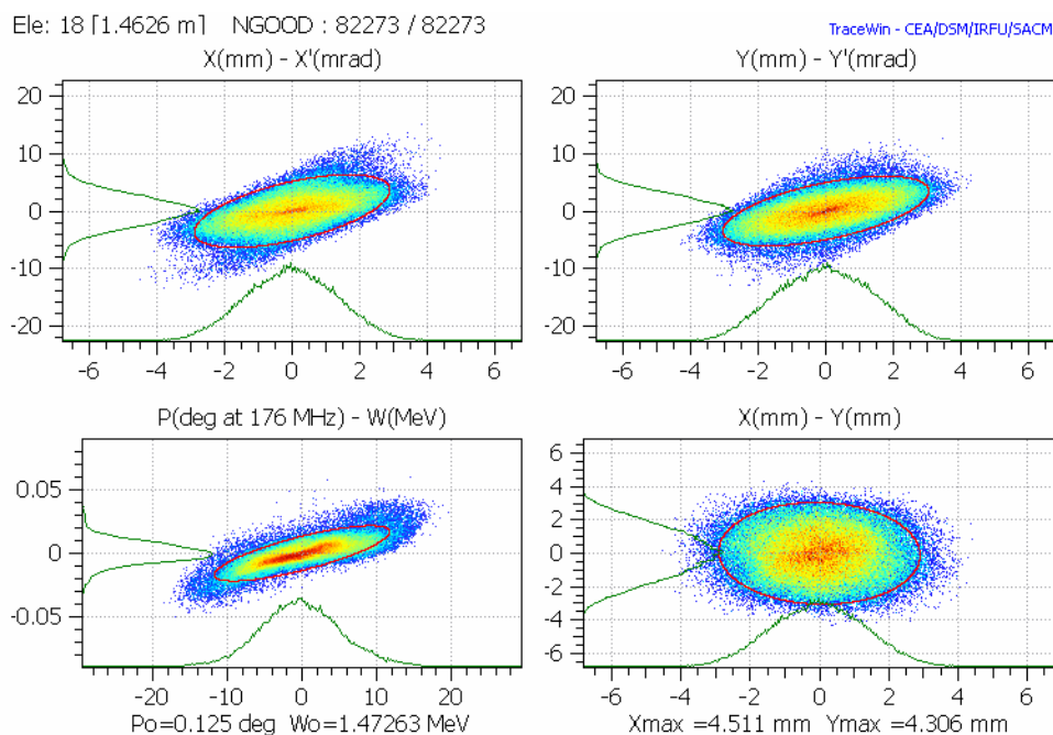
Fig. 4.5. H^- phase space distributions at the MEBT output (the scale is changed from the previous plots). The low energy tail is completely removed by the MEBT.
