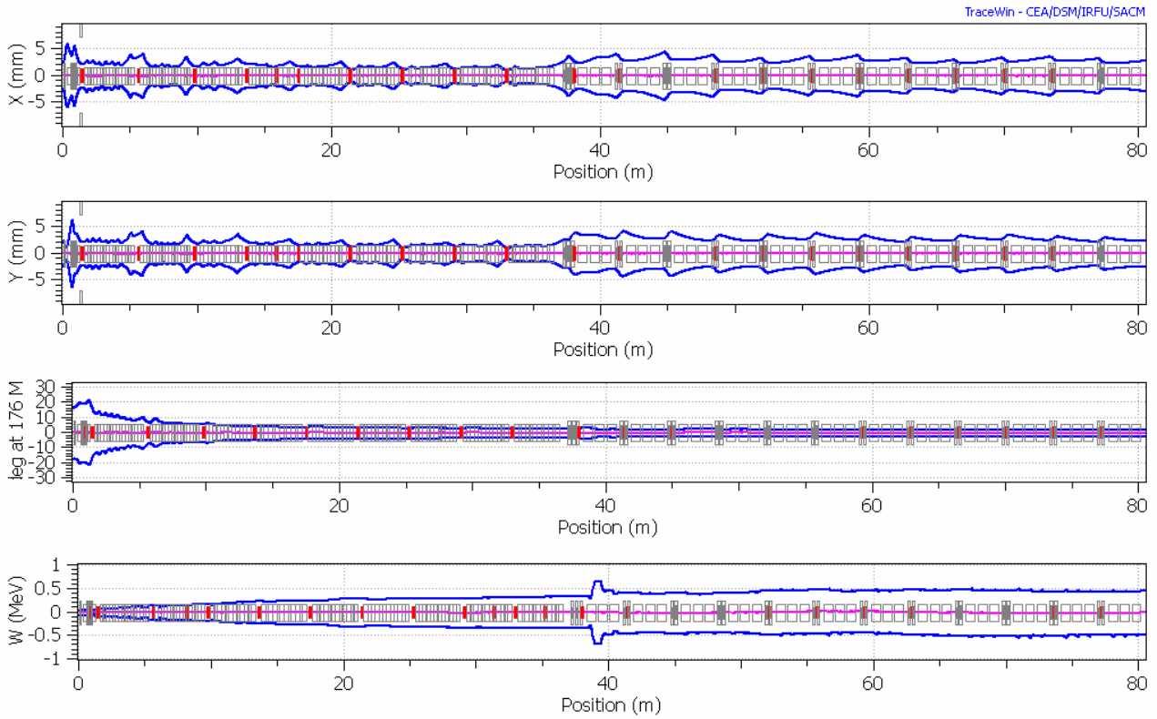
Fig. 4.16. 2 rms envelope for {}^3\text{He}^{++} .
