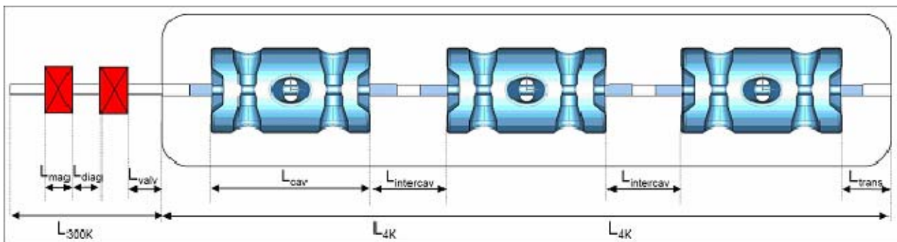
Fig. 3.8. Schematic layout of the \beta=0.3 cryomodule containing Spoke cavities. L_{\text{mag}}=200 mm; L_{\text{diag}}=130 mm; L_{\text{trans}}=223 mm; L_{\text{cav}}=538 mm; L_{\text{intercav}}=346 mm; L_{300K}=850 mm; L_{4K}=1868 mm.
