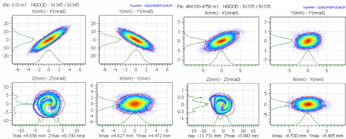
Figure 4.17. {}^3\text{He}^{++} phase space at the linac input (left) and output. 99% emittance ellipses in red.
