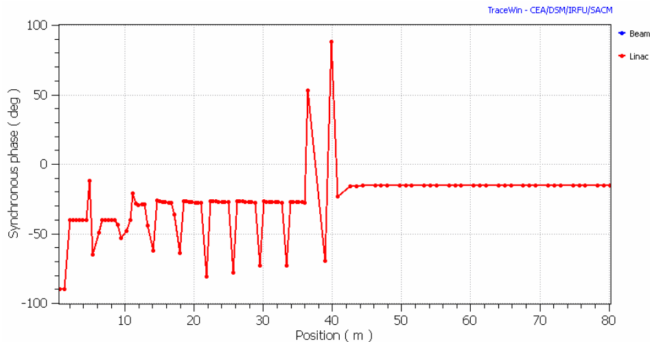
Fig. 4.2. H - beam synchronous phase profile in the LMB. The deviation from the nominal phase values are located in cavities used for bunching and matching purposes.
