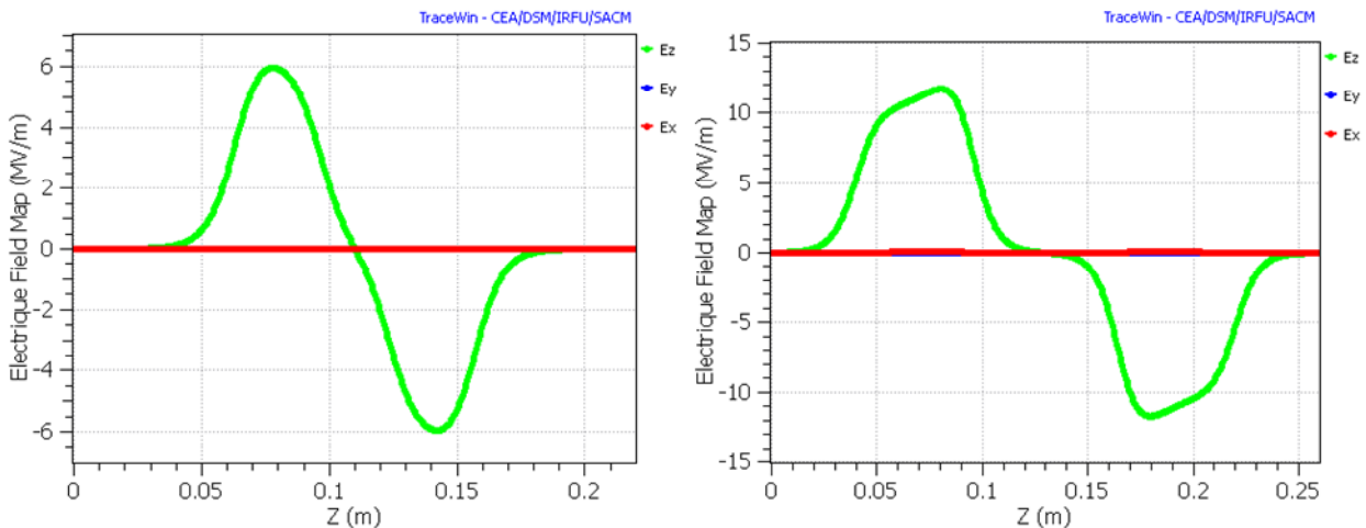
Figure 5.6. Accelerating field profile on axis in the \beta=0.09 (left) and \beta=0.16 HWR EURISOL cavities.
