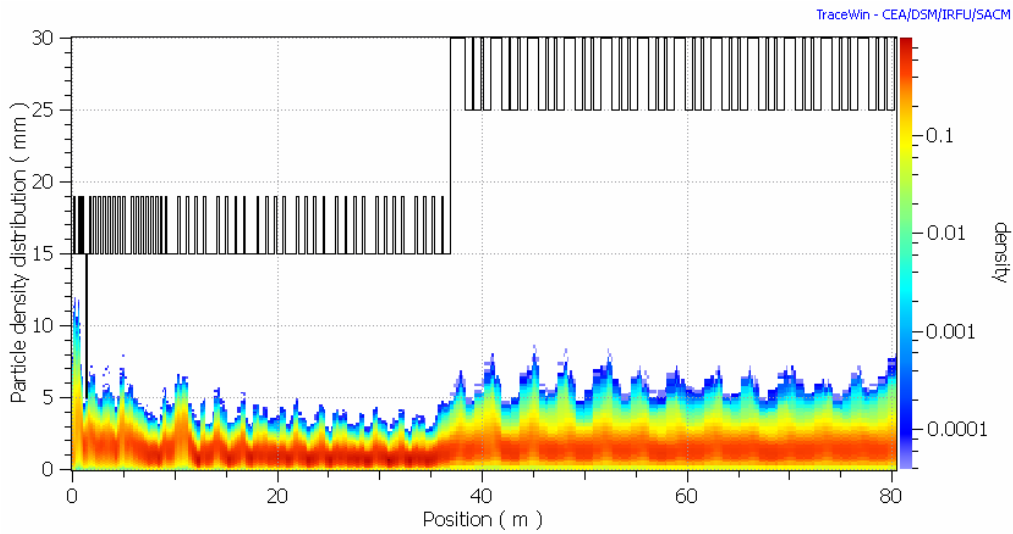
Fig. 4.10 Left: Particle density distribution along the linac for H. The black line represents the beam pipe aperture.
