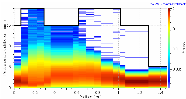
Fig. 4.6. H^- particle density distribution in the MEBT, showing that most of the low-energy tail is lost in the first half of the MEBT.
