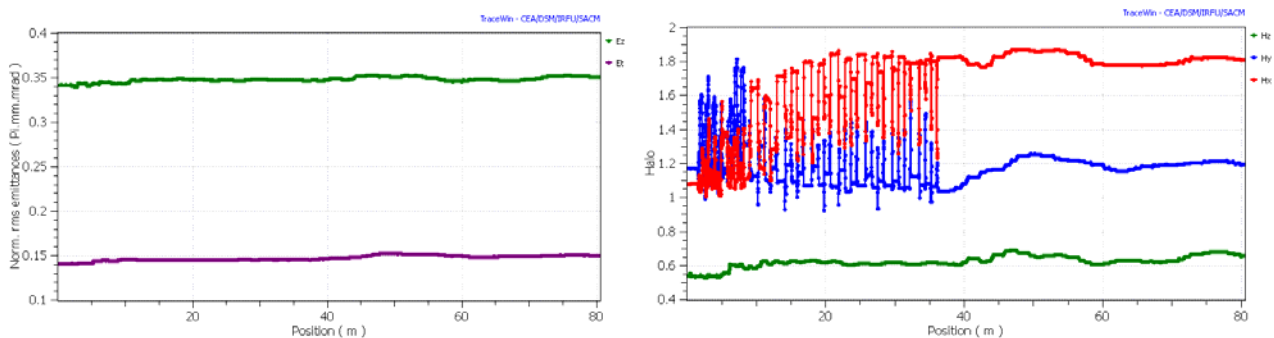
Figure 4.19. Emittance evolution (left) and halo parameter along the linac for ^3\text{He}^{++} .
