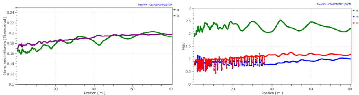
Figure 4.12. Normalized rms H^- beam emittance evolution (left) and halo parameter along the linac.
