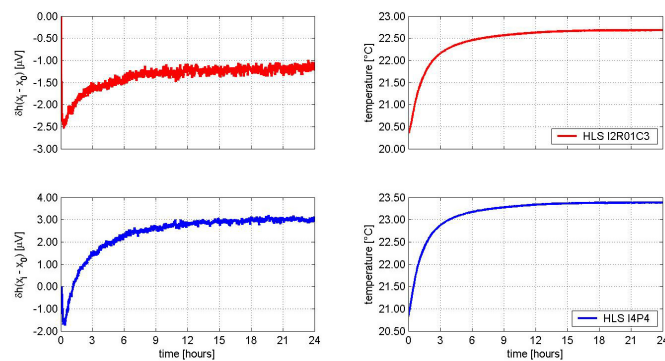
figure 8: warm up of HLS
