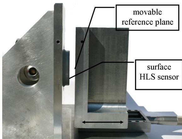
figure 5: side view of test bench
