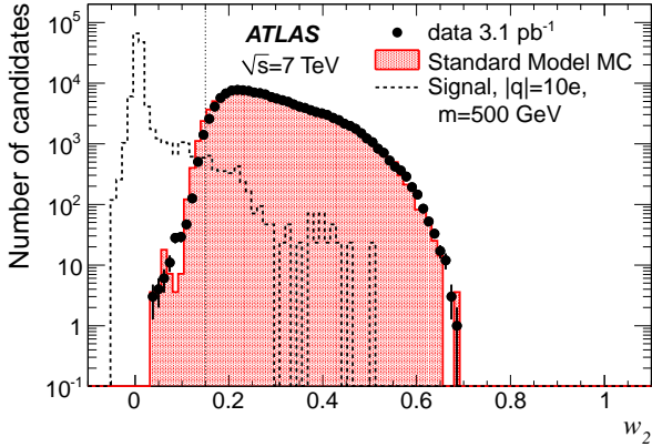
Figure 3: Distributions of w_1 and w_2 following the loose selection. Data (dots) are compared with area-normalised signal ( |q| = 10e and m = 500 GeV, dashed lines) and Standard Model background (shaded area) simulations. Negative values are caused by pedestal fluctuations. Dotted lines show the selection cut values.
