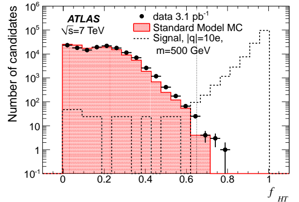
Figure 2: Distribution of the fraction of TRT high-threshold hits for candidates satisfying the loose selection. Data (dots) are compared with area-normalised signal ( |q| = 10e and m = 500 GeV, dashed line) and Standard Model background (shaded area) simulations. The dotted line shows the selection cut value.
