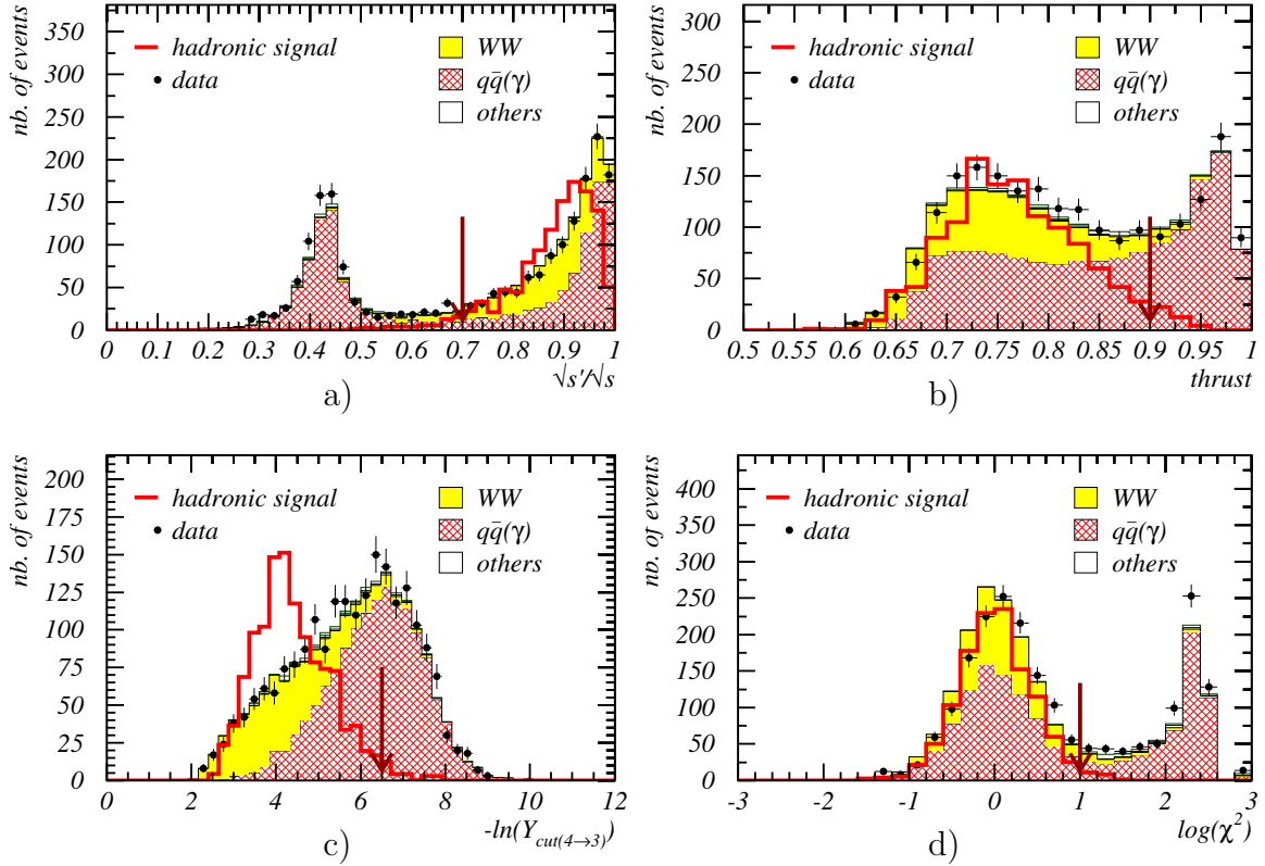
Figure 4: Distributions of variables relevant for the sequential selection of the hadronic topology are shown at \langle\sqrt{s}\rangle = 206.6 GeV: a) ratio between the effective centre-of-mass energy and the centre-of-mass energy; b) thrust; c) -\ln(y_{4\to 3}) ; d) \chi^2 of the kinematic fit imposing energy-momentum conservation. The WW, q\bar{q}(\gamma) and “others” labels represent the background contribution from charged-current four-fermion final states generated with WPHACT [22–24], two-fermion final states generated with KK2F [26] and all the other processes mentioned in Section 3, respectively. The signal normalisation is arbitrary, but the same in all plots. The arrows show the applied cuts.
