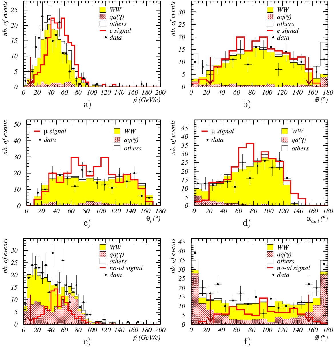
Figure 5: Distributions of variables relevant for the sequential selection of the semi-leptonic topology after the common preselection are shown at \langle\sqrt{s}\rangle = 206.6\text{ GeV} . e sample: a) missing momentum; b) polar angle of the missing momentum (after applying the cut on the missing momentum distribution); \mu sample: c) lepton polar angle; d) lepton isolation angle; no-id sample: e) missing momentum; f) polar angle of the missing momentum (after applying the cut on the missing momentum distribution). The WW, q\bar{q}(\gamma) and “others” labels have the same meaning as in Fig. 4. The signal normalisation is arbitrary, but the same in all plots. The arrows show the applied cuts.
