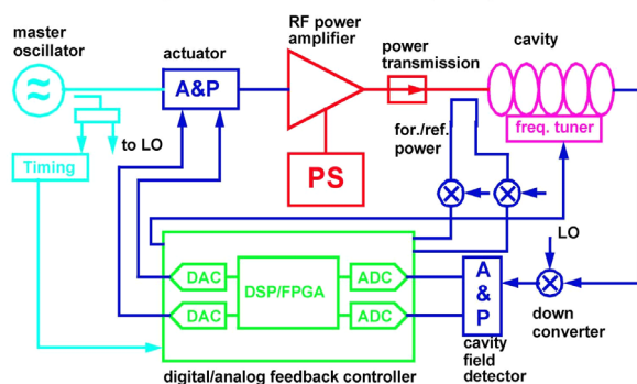
Figure 1: LLRF system architecture.
