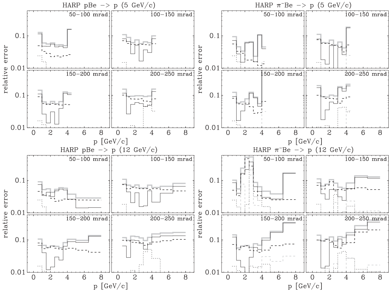
FIG. 2. Total systematic error (grey solid line) and main components for a typical (Be) target with incident p and \pi^- beams at 5 and 12 GeV/c: black short-dashed line for absorption + tertiary interactions, black dotted line for track efficiency and target pointing efficiency, black solid line for momentum scale + resolution and angle scale, grey short-dashed line for PID.
