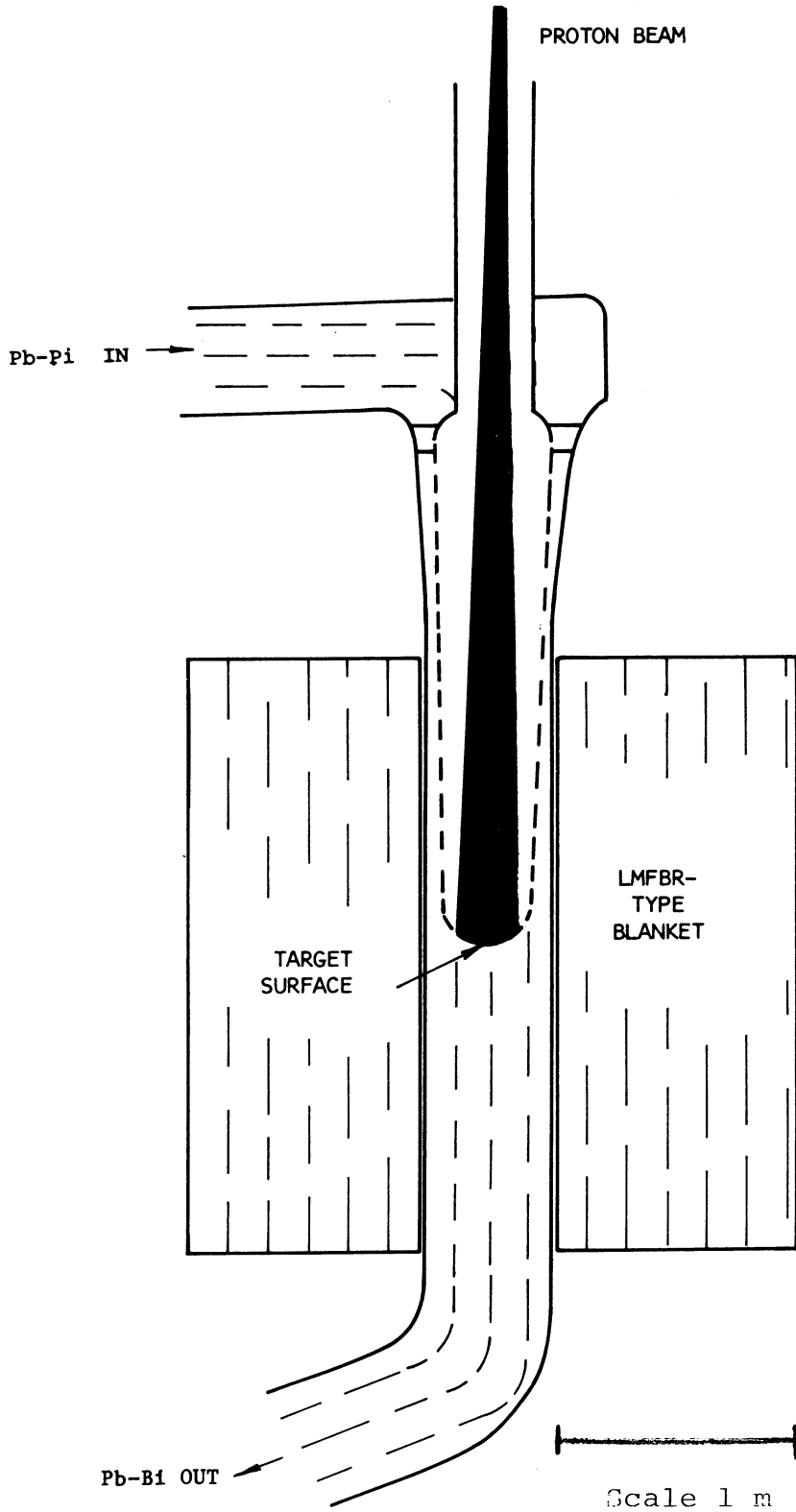
Fig. 5 Schematic diagram of a windowless target of liquid metal surrounded by a liquid-metal cooled blanket.
