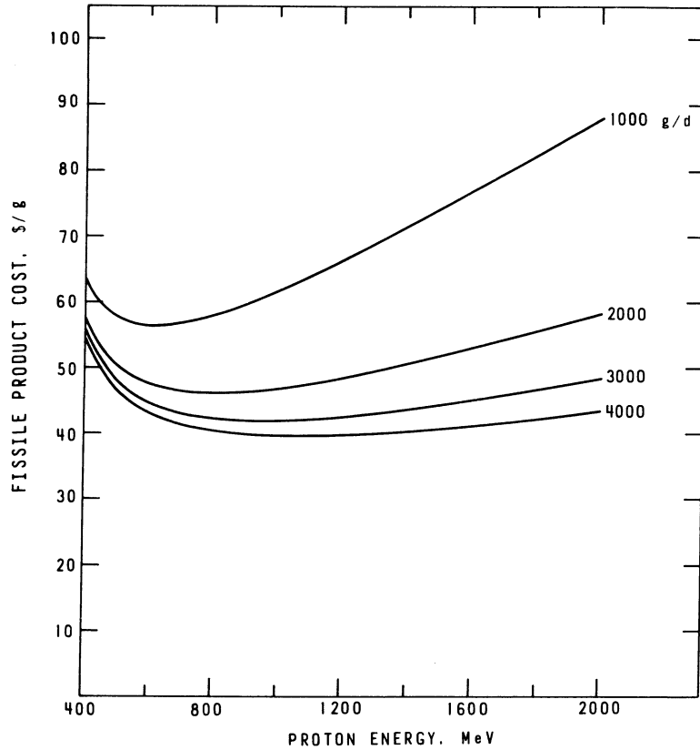
Fig. 3 Calculated unit fissile product costs for production rates 1000 to 4000 grams per day vs. proton energy. The principal assumptions are: electrical power costs, $0.007/(kW·h); target costs included in the electrical power costs; interest and depreciation, 10% per year; rf equipment capital $350/kW; accelerator unit length cost, $60,000/m; maximum peak accelerating field, 2 MV/m, averaged over the accelerator length.
