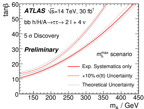
Figure 2. 5\text{-}\sigma discovery contour for ll -channel of b\bar{b} h/H/A \rightarrow \tau\tau as a function of m_A and \tan\beta for an integrated luminosity of 30 \text{ fb}^{-1} .
