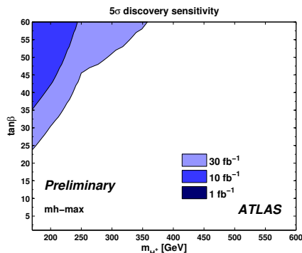
Figure 5. Discovery contour in the m_h - \max scenario for gg/gb \rightarrow t[b]H^+ \rightarrow bqq[b]\tau_{had}\nu . Systematic and statistical uncertainties are included. The systematic uncertainty is assumed to be 10% for the background, and 44% for the signal. The lines indicate a 5\sigma significance for the discovery.
