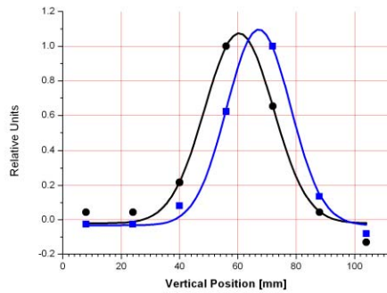
Figure 2: Single pass beam profile of a pulsed (1.35 GeV, p=10 mbar) normal positioned (●) and shifted (■) beam (Gaussian fit to PMT data).
