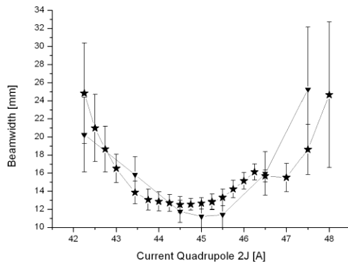
Figure 5: Horizontal \sigma -beam widths versus quadrupole strength for a 3.14 MeV proton beam.
