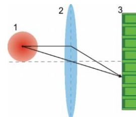
Figure 1: Measurement Principle (not to scale): The light from the beam (1) is focused with a glass lens (2) onto the multichannel photomultiplier (3).
