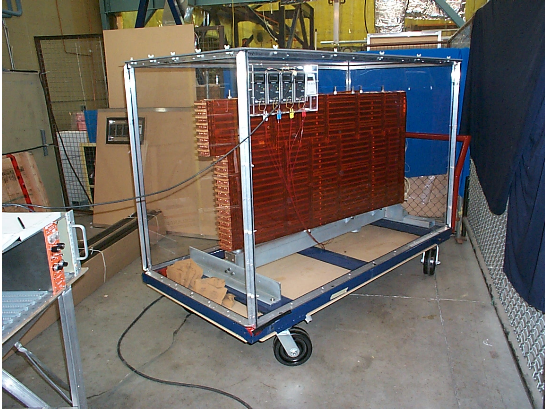
Figure 9: Module undergoing a long term HV test at 1800 V for 10 days. The module is bolted on its shipping frame, and stored in a clean area or box. The relative humidity is monitored as well as the currents in the liquid argon subgaps.
