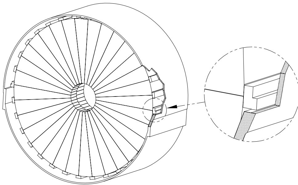
Figure 3: Schematic of the support of the HEC within the end-cap cryostat. The outer radius of the HEC (warm) is 2.09 m.
