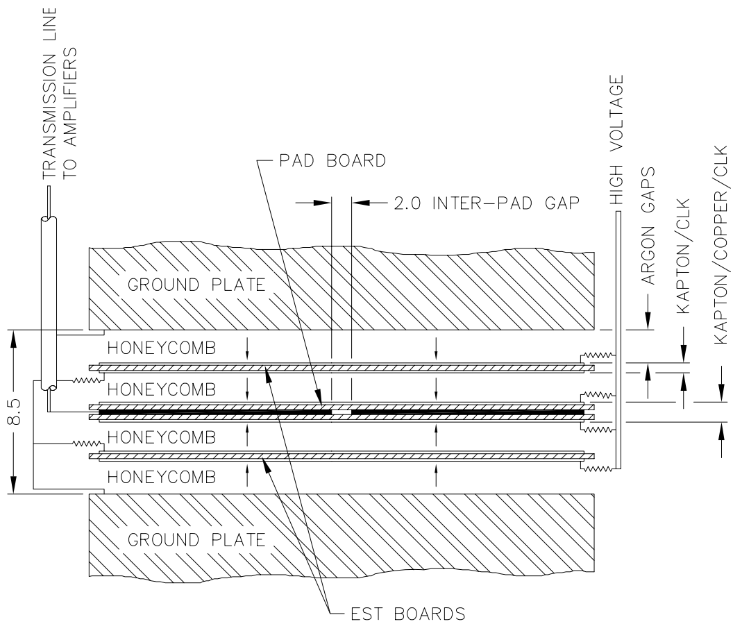
Figure 4: Schematic of the arrangement of the read-out structure in the 8.5mm inter-plate gap. Dimensions are in mm.
