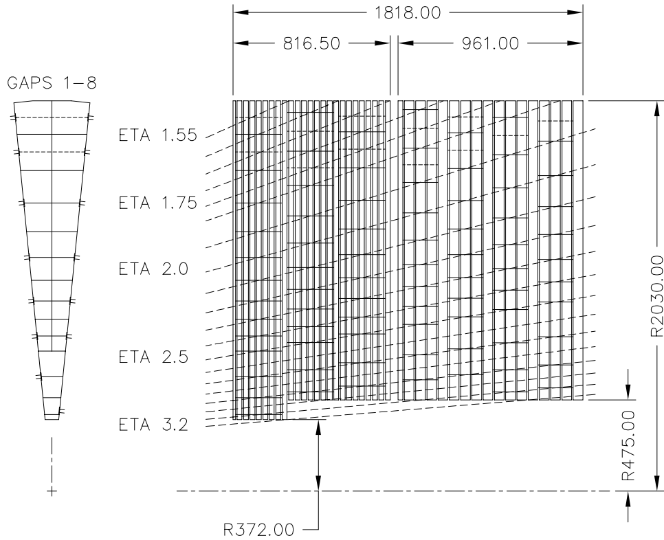
Figure 2: Schematic r-\phi (left) and r-z (right) view of the hadronic end-cap calorimeter modules. Note the semi-pointing layout of the read-out electrodes, as indicated by the dashed lines. Units are in mm.
