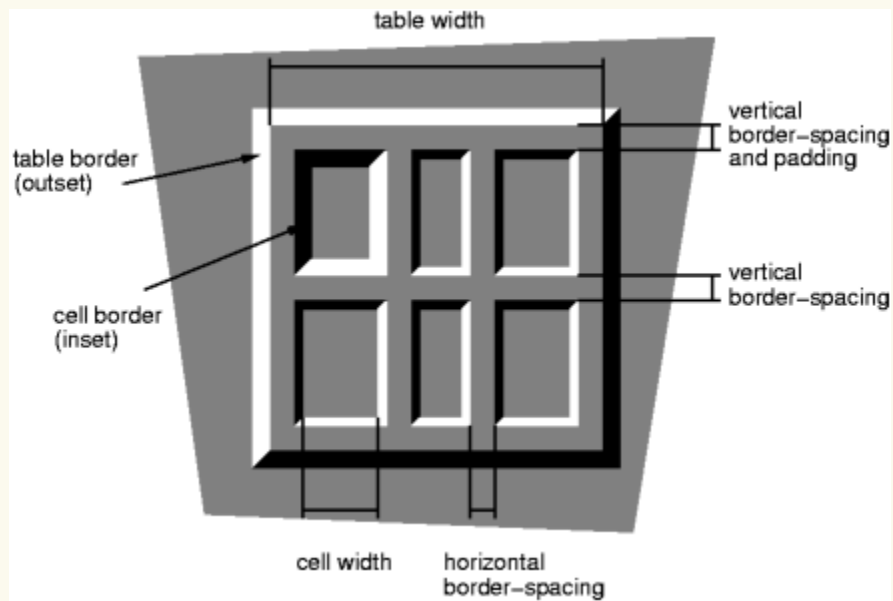
A table with 'border-spacing' p.317 set to a length value. Note that each cell has its own border, and the table has a separate border as well.
