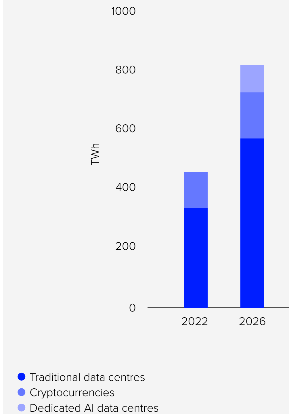
Figure 23. Electricity demand from data centres, AI and cryptocurrency 2022 and 2026
