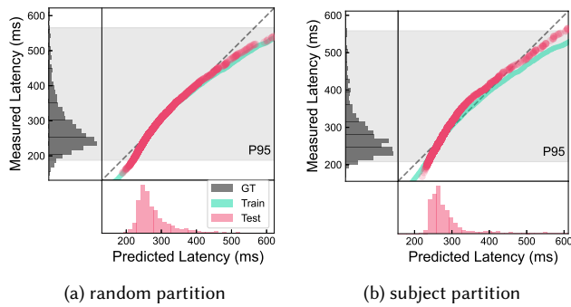
Fig. 6. Model performance and generalization validation using preliminary user study dataset. Q-Q plots for various train/test splits demonstrate our model’s accuracy and ability to generalize when applied to new data. In each plot, we visualize a comparison of histograms between the ground truth data (gray), and the model predictions on the test dataset (magenta). We also visualize the baseline Q-Q plot for the model’s performance on the training dataset in (teal). The P95 confidence interval is highlighted in each figure to contextualize the volume of data being shown. As defined in Section 6.1, (a) shows the results with random partition (1). (b) shows the results with subject_01’s data partition (2). We observe a distribution agreement between our model prediction and the unseen testing dataset; the closer the Q-Q curves are to the diagonal line, the more accurate the predictions are. The corresponding K.S. tests evidence the observation.
