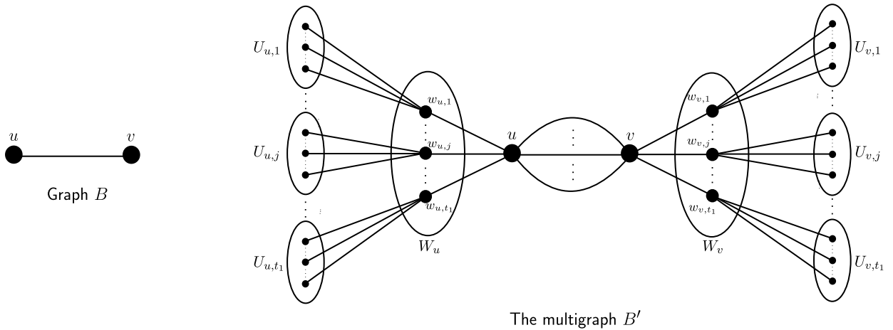
Fig. 1. An illustrative diagram of the reduction in the proof of Lemma 12. As an example, we consider the (bipartite) graph B in the left part of the picture to be the input to #BIS. The respective input B' to BI-M-NONUNIFORM-2-SPIN( \alpha, \alpha, \lambda ) is shown in the right part of the picture. For this graph B , where \deg(u) = \deg(v) = 1 , t_1 is the number of parallel edges between u and v in B' , as well as the cardinalities of the sets W_u and W_v (where t_1 is an appropriate integer, cf. (6)). Also, t_2 (cf. (7)) equals the cardinalities of the sets U_{u,j} and U_{v,j} for j = 1, \dots, t_1 . For a general graph B and a vertex u in B , the cardinality of the set W_u depends on the degree of the vertex u and equals t_1 \deg(u) . Other than that, the construction of the multigraph B' is analogous by iterating the construction in the figure for each edge in B .
