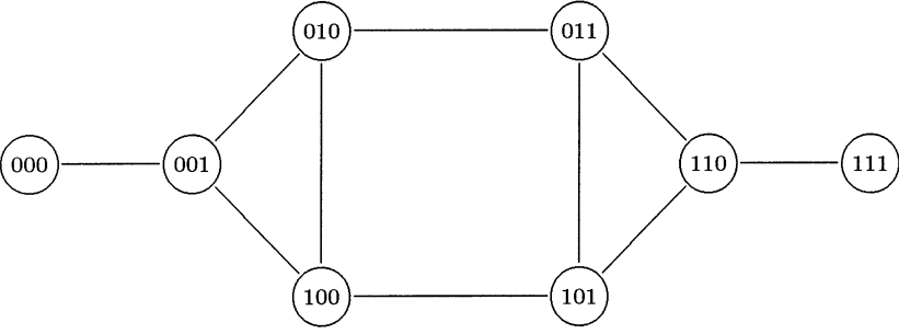
Fig. 1. Graph SE(3) .
