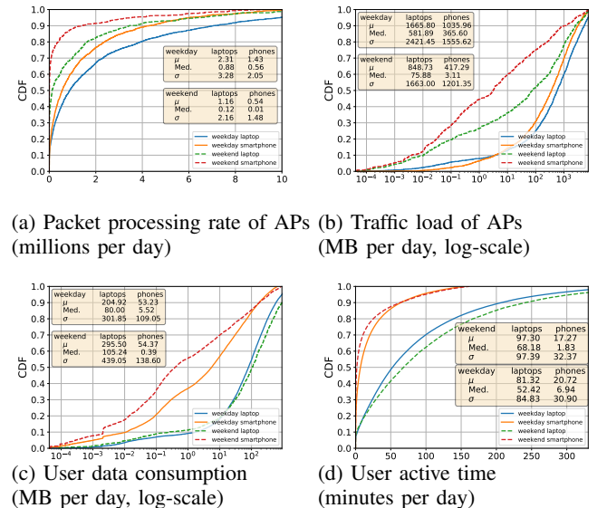
Fig. 7: Distribution plots
