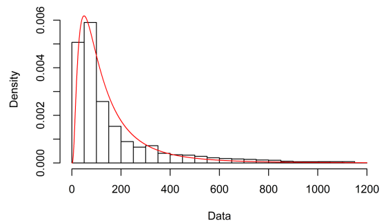
Fig. 15: Lognormal distribution.
