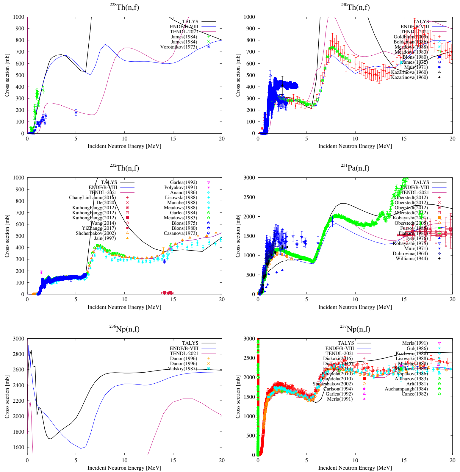
Figure 6.6: Fission cross sections for Th, Pa and Np isotopes.
