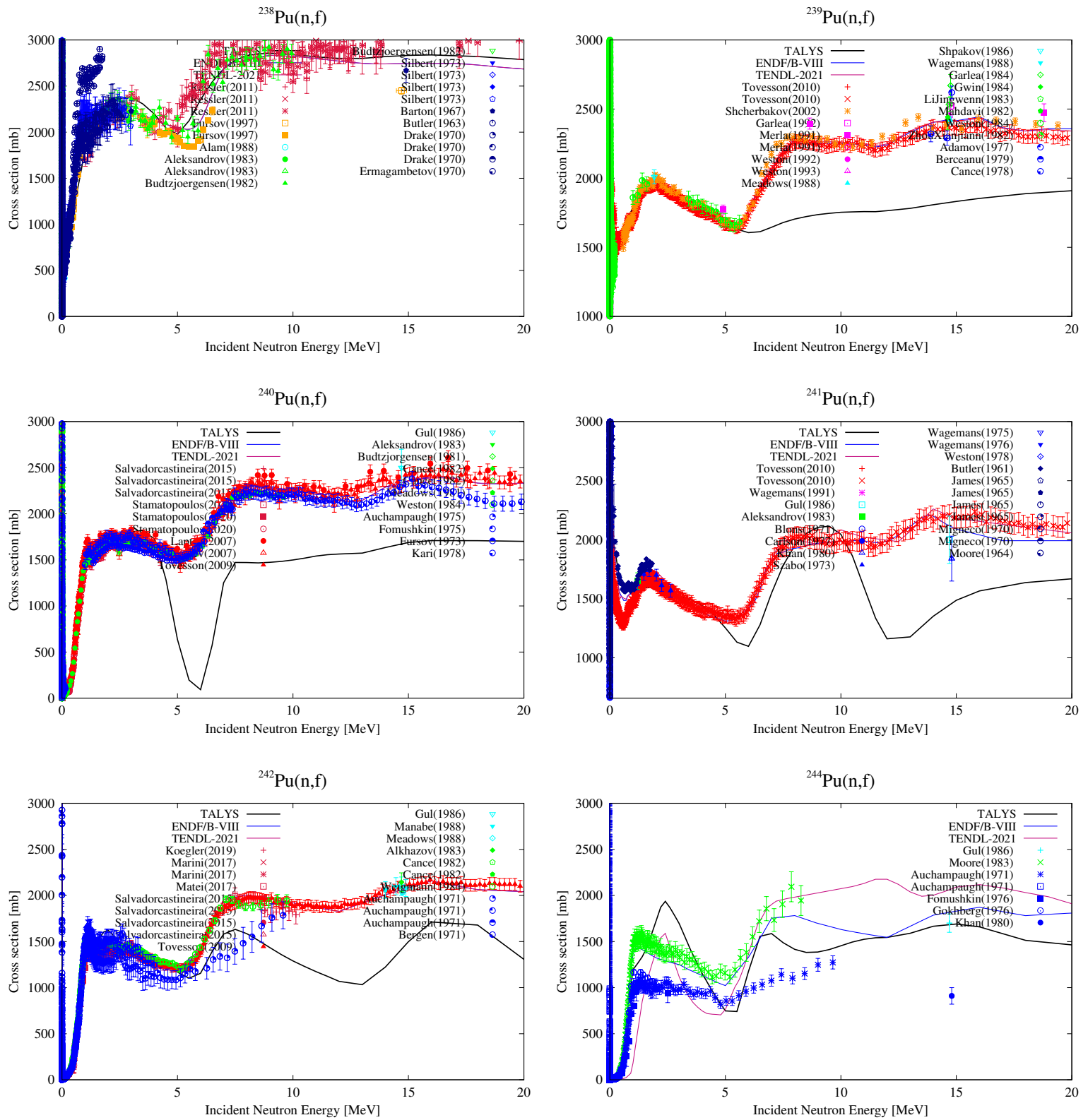
Figure 6.8: Fission cross sections for Pu isotopes.
