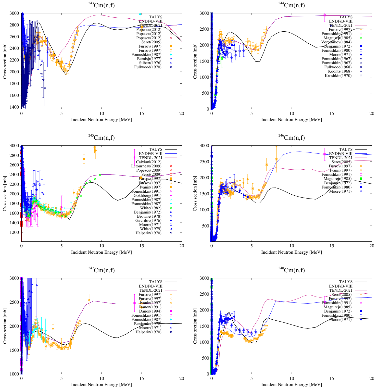
Figure 6.9: Fission cross sections for Cm isotopes.
