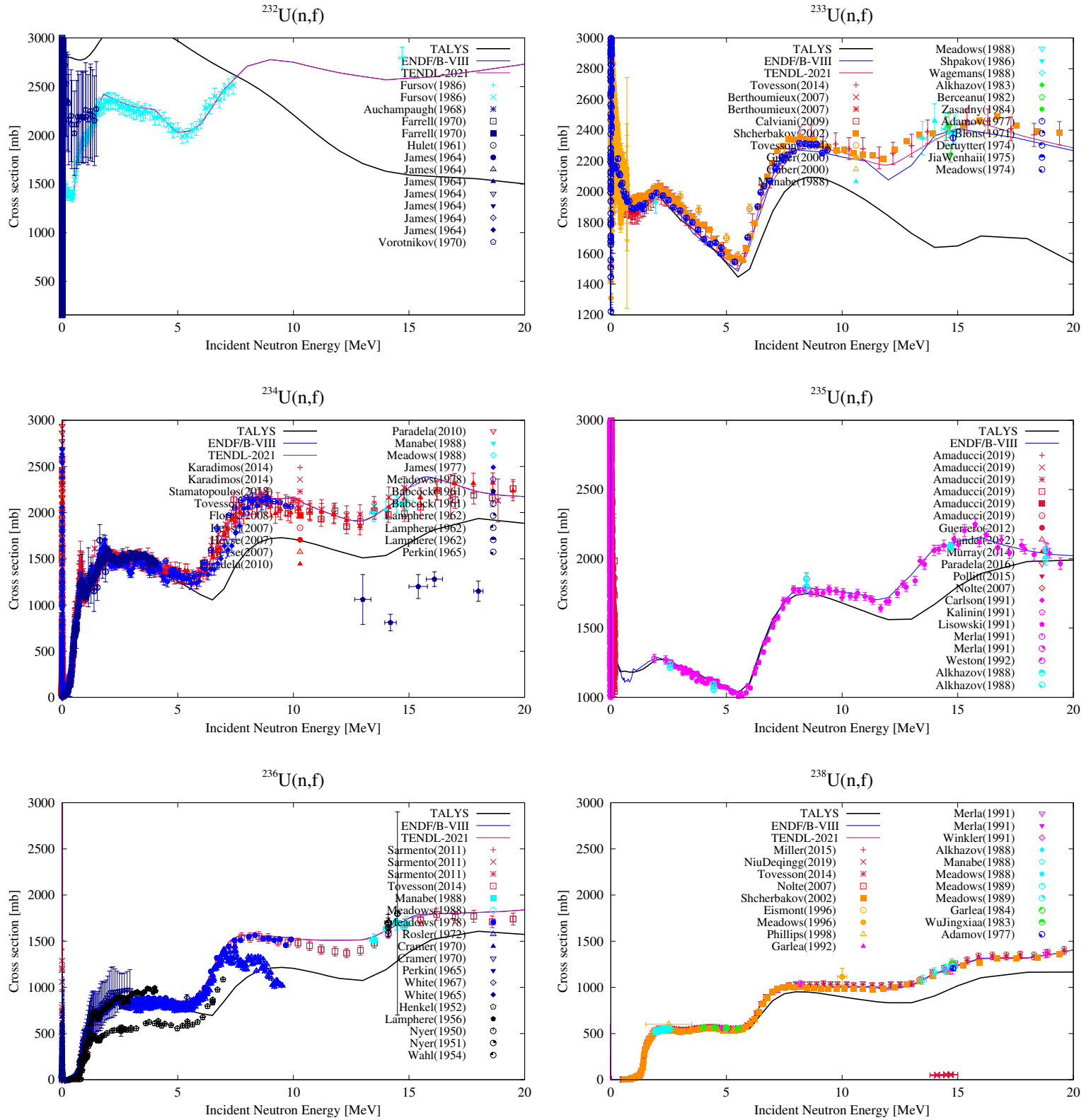
Figure 6.7: Fission cross sections for U isotopes.
