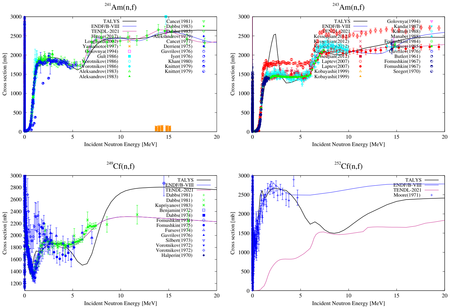
Figure 6.10: Fission cross sections for Am, Bk and Cf isotopes.
