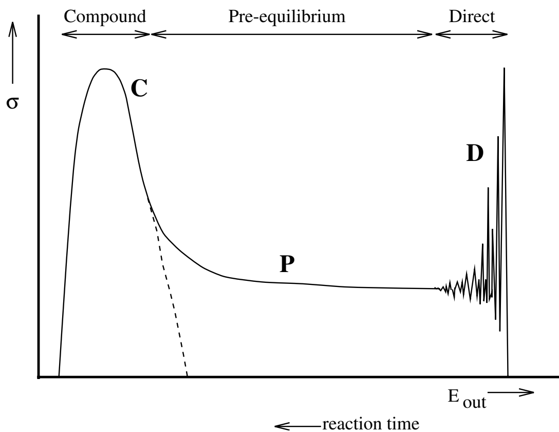
Figure 4.2: Schematical drawing of an outgoing particle spectrum. The energy regions to which direct (D), pre-equilibrium (P) and compound (C) mechanisms contribute are indicated. The dashed curve distinguishes the compound contribution from the rest in the transitional energy region.
