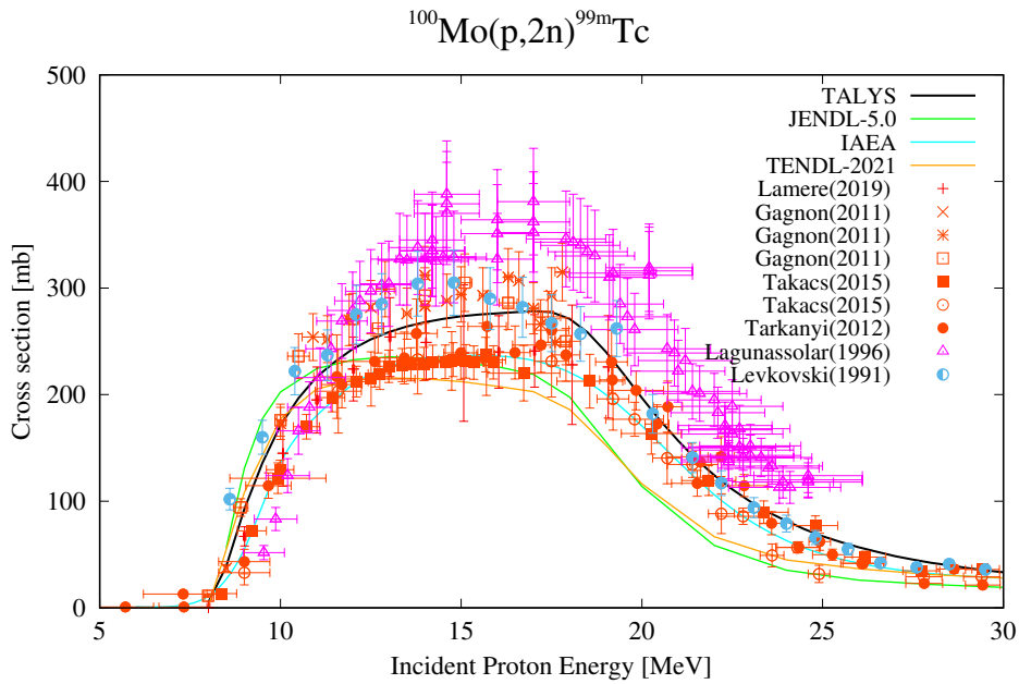
Figure 19.1: Excitation function of ^{100}\text{Mo}(p,2n)^{99m}\text{Tc} .
