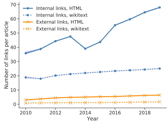
Figure 3: Number of links extracted from wikitext and HTML, averaged over 404K articles created in 2009; 95% error bands estimated via bootstrap resampling.
