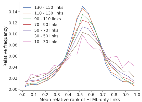
Figure 5: Histograms of mean relative rank of HTML-only links among all HTML links in terms of click frequency, averaged over 405K articles. One curve per out-degree bracket.
