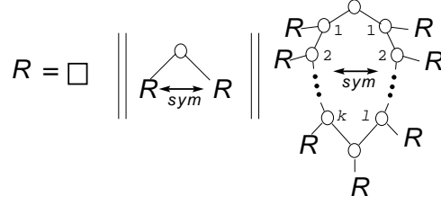
Figure 4: Symbolic specification of normal galled trees.
