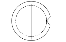
Figure 2: The domain where we require analyticity.
