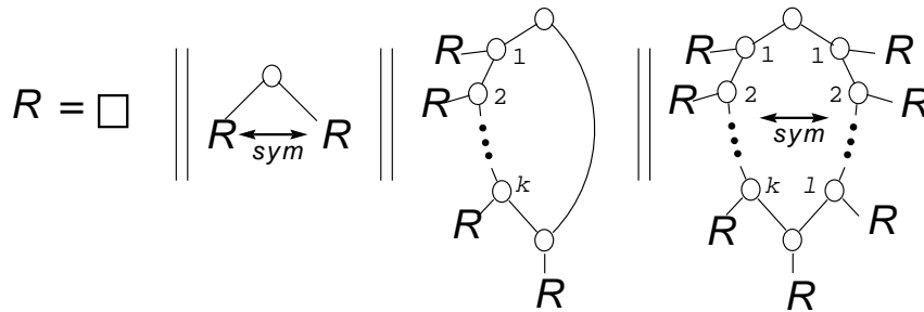
Figure 1: Symbolic specification of galled trees.
