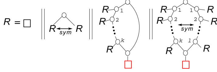
Figure 3: Symbolic equation for simplex galled trees. The red substructures are the places where galled trees and simplex galled trees differ.
