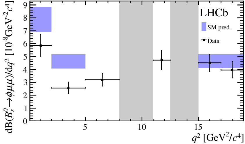
Figure 4: Differential branching fraction of the decay B_s^0 \rightarrow \phi\mu^+\mu^- , overlaid with SM predictions [4, 5] indicated by blue shaded boxes. The vetoes excluding the charmonium resonances are indicated by grey areas.
