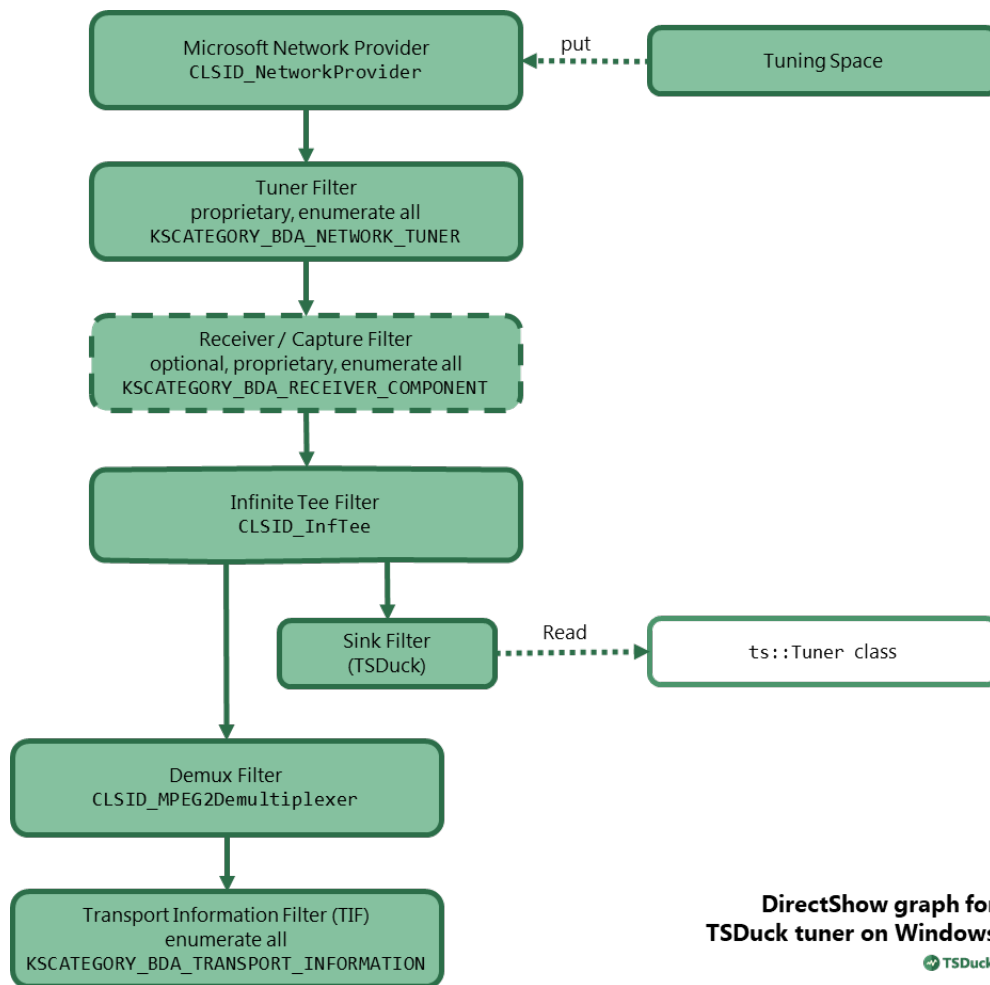
Figure 3. Usage of Windows DirectShow interfaces in TSDuck
