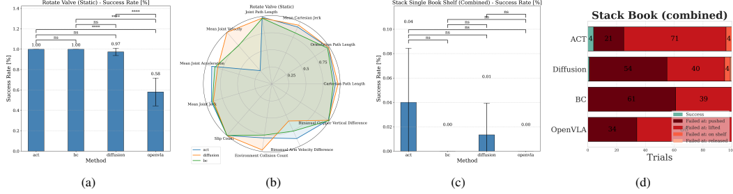
Figure 7: Behavioral and outcome metrics provide complementary insights across task difficulties. (a) Success rates for an easy task (Rotate Valve (static)) show ceiling effects, masking performance differences. (b) Behavioral metrics reveal Diffusion Policy’s superior motion quality despite identical success. (c) In a hard task (Stack Single Book Shelf (combined)), uniformly low success rates offer little insight. (d) Stagewise failure analysis highlights push-to-edge and lifting stages as key bottlenecks, exposing specific policy shortcomings.
