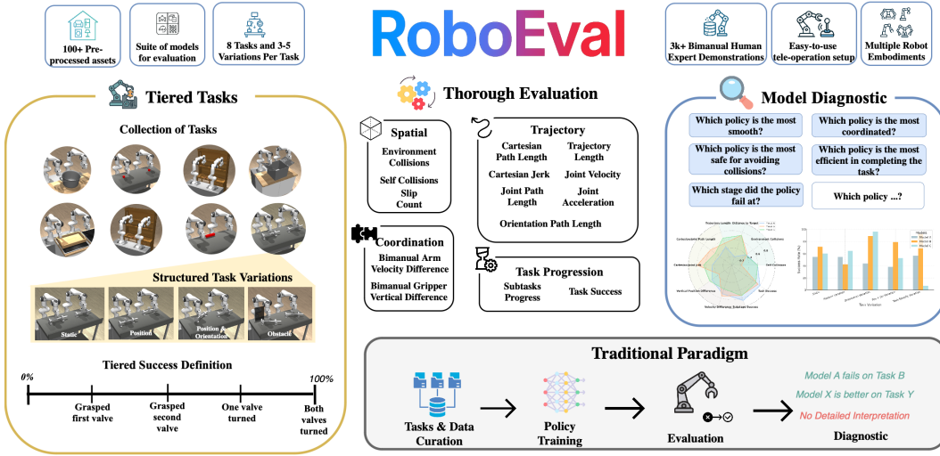
Figure 1: Overview of ROBOEVAL. ROBOEVAL is a structured and scalable simulation benchmark for bimanual manipulation, featuring 3,000+ human-collected demonstrations across 8 tasks, each with 3-5 variations. It includes a standardized asset library—collision meshes, annotated sites, and manipulable objects—for building and augmenting tasks with spatial perturbations and distractors. A VR-based teleoperation interface enables realistic data collection. For analysis, ROBOEVAL provides rich evaluation tools that go beyond binary success, measuring task progression, coordination, trajectory efficiency, and spatial proximity.
