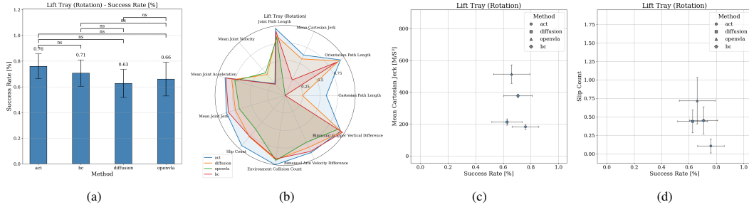
Figure 4: Behavioral metrics differentiate policies with similar success rates. (a) Bar plot of success rates for the Lift Tray (Rotation) task, where no statistically significant differences are observed across policies. (b) Radial plot comparing policies along multiple behavioral metric dimensions, with values normalized and polarity-adjusted to fall within [0, 1] such that higher values indicate better performance. (c) Scatter plot showing the mean Cartesian jerk per policy. (d) Scatter plot showing the mean slip count per policy. Error bars represent 95% confidence intervals; ‘ns’ denotes comparisons with p > 0.05 .
