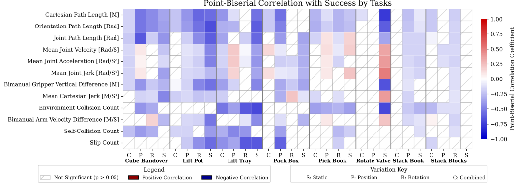
Figure 3: Point-Biserial Correlation Between Behavioral Metrics and Trajectory Success. We compute the point-biserial correlation between each behavioral metric and binary trajectory success across different task variations, highlighting only statistically significant correlations. Rows are sorted by the number of significant correlations per metric (descending), placing metrics most consistently associated with success at the top. Overall, 59.4% of metric-task pairs show statistically significant correlation, indicating that behavioral metrics are meaningfully related to success in the majority of tasks.
