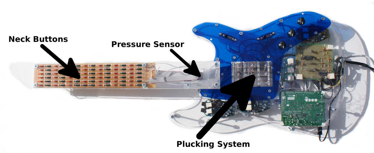
Figure 2. Top view of the BLADEAXE.
