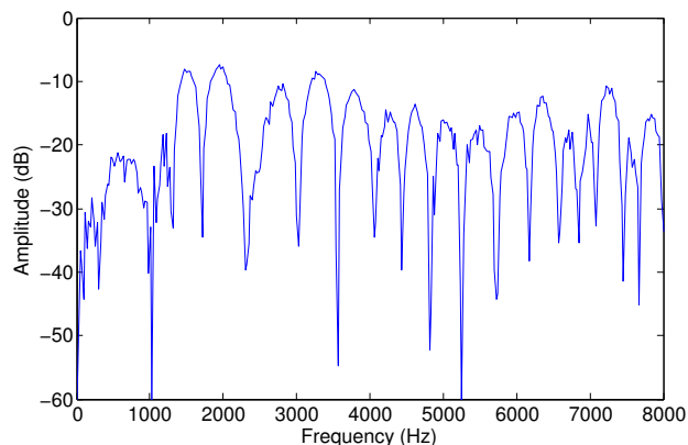
Figure 5. Fast Fourier Transform of the signal of the pulse presented in figure 4.
