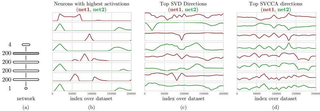
Figure 1: To demonstrate SVCCA, we consider a toy regression task (regression target as in Figure 3). (a) We train two networks with four fully connected hidden layers starting from different random initializations, and examine the representation learned by the penultimate (shaded) layer in each network. (b) The neurons with the highest activations in net 1 (maroon) and in net 2 (green). The x-axis indexes over the dataset: in our formulation, the representation of a neuron is simply its value over a dataset (Section 2). (c) The SVD directions — i.e. the directions of maximal variance — for each network. (d) The top SVCCA directions. We see that each pair of maroon/green lines (starting from the top) are almost visually identical (up to a sign). Thus, although looking at just neurons (b) seems to indicate that the networks learn very different representations, looking at the SVCCA subspace (d) shows that the information in the representations are (up to a sign) nearly identical.
