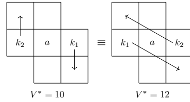
Figure 5: An example of two Grid states that are considered isomorphic by the 1-WL algorithm with respect to the goal. The goal is to move the keys k_1 and k_2 to specific cells, as the arrows indicate. All keys and locks have the same shape. The agent a is in the center of the grid. In the left state, 10 actions are needed to solve the instance, while 12 actions are needed in the right state.
