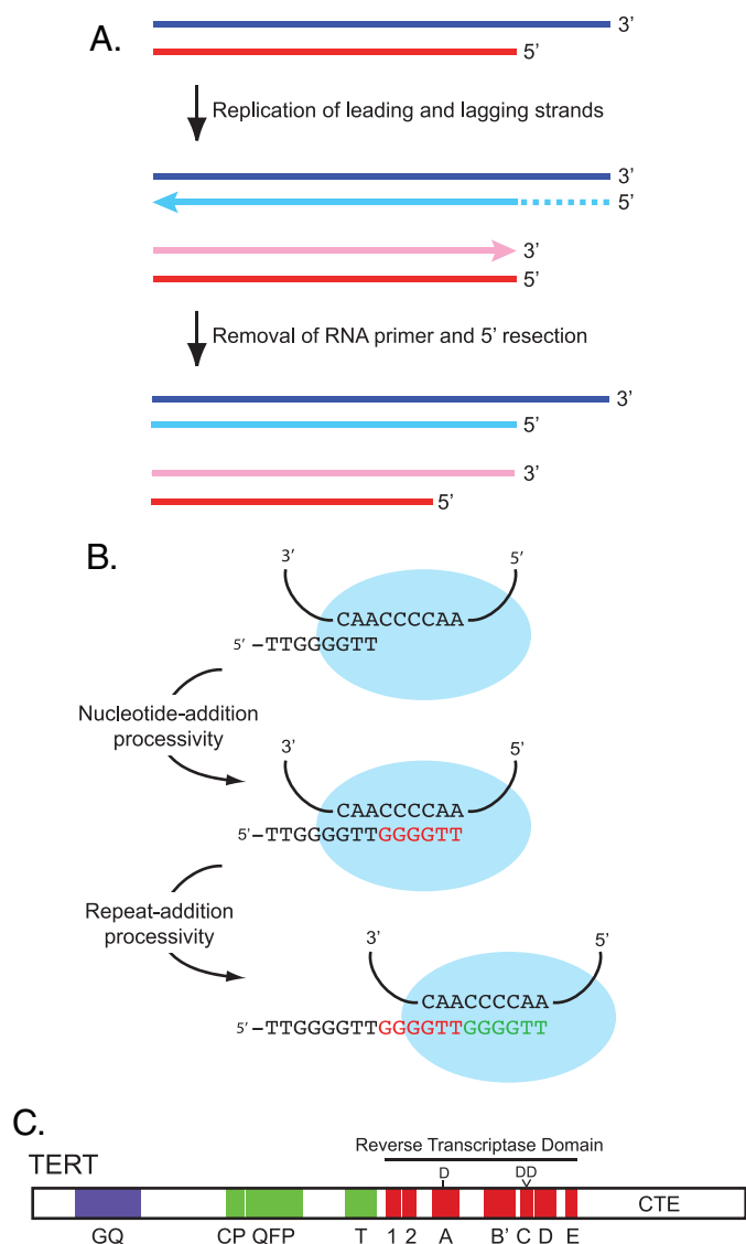
FIGURE 1. The end replication problem and telomerase. A , end replication problem. Replication of a telomere containing a 3'-overhang on the lagging-strand template (dark blue) and a recessed 5' terminus on the leading-strand template (red) is diagrammed. The RNA primer is depicted as a dotted line. B , general model of telomerase function. The template of the telomerase RNA (CA-rich sequence; shown from Tetrahymena ) is complementary to the 3'-terminal overhang. TERT protein (blue oval) adds nucleotides (red) until the template boundary is reached. Translocation and repositioning of the 3' terminus allow addition of a second repeat (green). C , generalized domain structure of TERT. Conserved aspartic acid residues (D) necessary for catalysis are indicated. The N terminus contains regions that confer high affinity (green) and low affinity (blue) RNA binding. For details, see Ref. 19.
