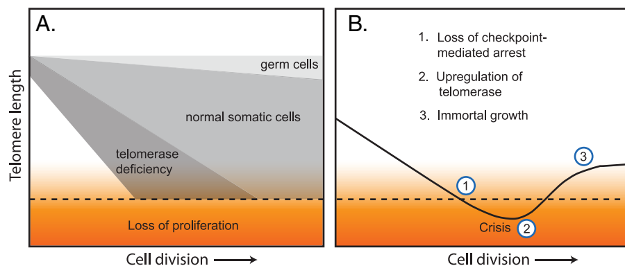
FIGURE 2. Telomere dynamics during normal and abnormal cell growth. A , in general, germ cells express telomerase and maintain long telomeres (light gray), whereas absent or low expression of telomerase in somatic cells and adult stem cells is insufficient to prevent telomere shortening (medium gray). Cell proliferation slows or ceases when cell cycle checkpoints are activated by short telomeres (dashed line), perhaps contributing to normal aging. Individuals with reduced telomerase activity exhaust telomere reserves more rapidly (dark gray), leading to premature aging, particularly in highly proliferative tissues. B , shown is a model of telomerase activation during tumorigenesis. When cell cycle checkpoints fail, cells divide in the face of severe telomere loss. Telomere uncapping causes genome instability and lethality (crisis). Reactivation of telomerase (or initiation of ALT) allows cells to exit crisis and proliferate with short but stable telomeres.
