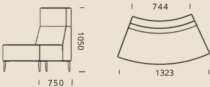
OAS-MB-45CVX
