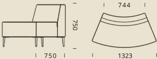
OAS-SB-45CVX
