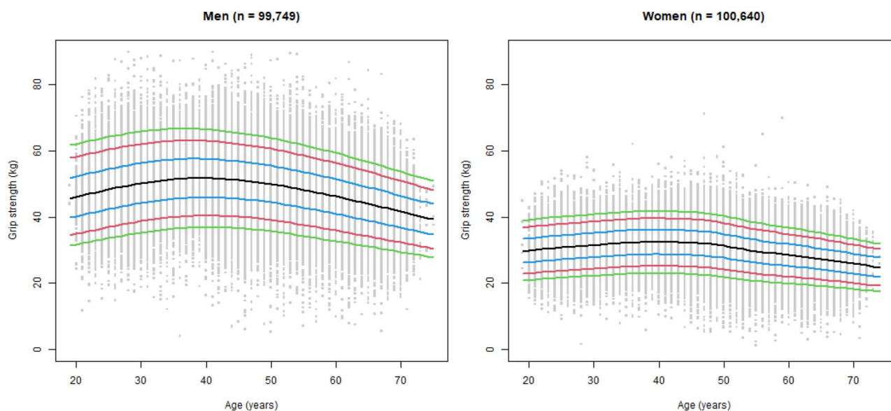
Figure 1. Percentile curves of grip strength across age for men and women in the NAKO sample. The 5th (green), 10th (red), 25th (blue), 50th (black), 75th (blue), 90th (red) and 95th (green) percentiles of grip strength (kg) across age (years) are presented for men (left) and women (right). n: number of participants.
