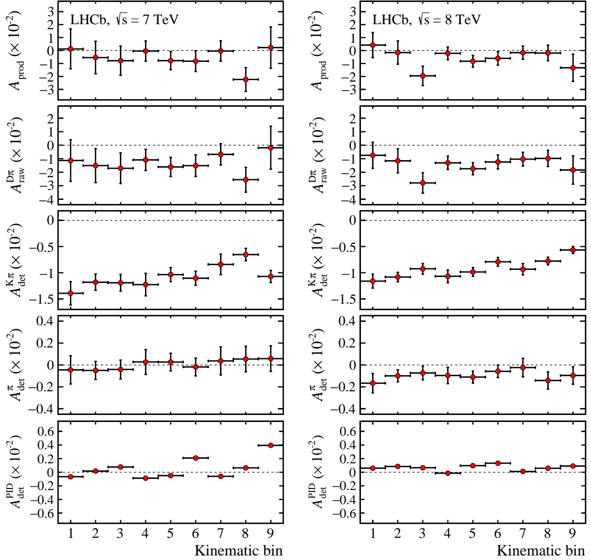
Figure 1: A summary of the individual asymmetry terms that go into the computation of the production asymmetries in (left) the 7 TeV and (right) 8 TeV datasets. The upper sub-figures show the \mathcal{A}_{\text{prod}} values.
