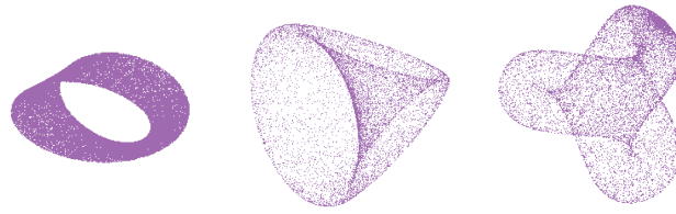
Figure 8: Möbius strip, Steiner’s roman surface, and Boy’s surface.
