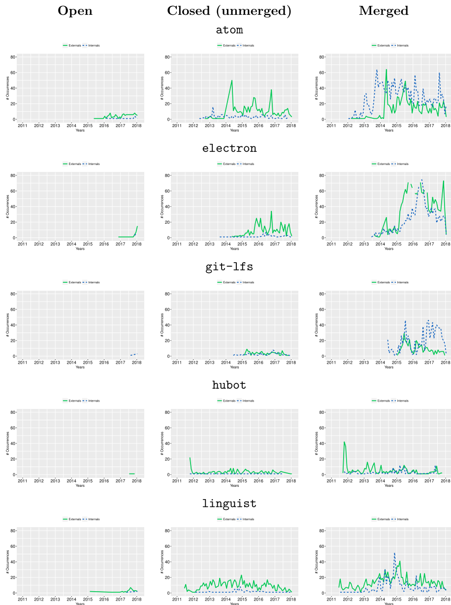
Fig. 2 Time series for open, closed/merged, and closed/unmerged pull requests submitted by internals and externals
