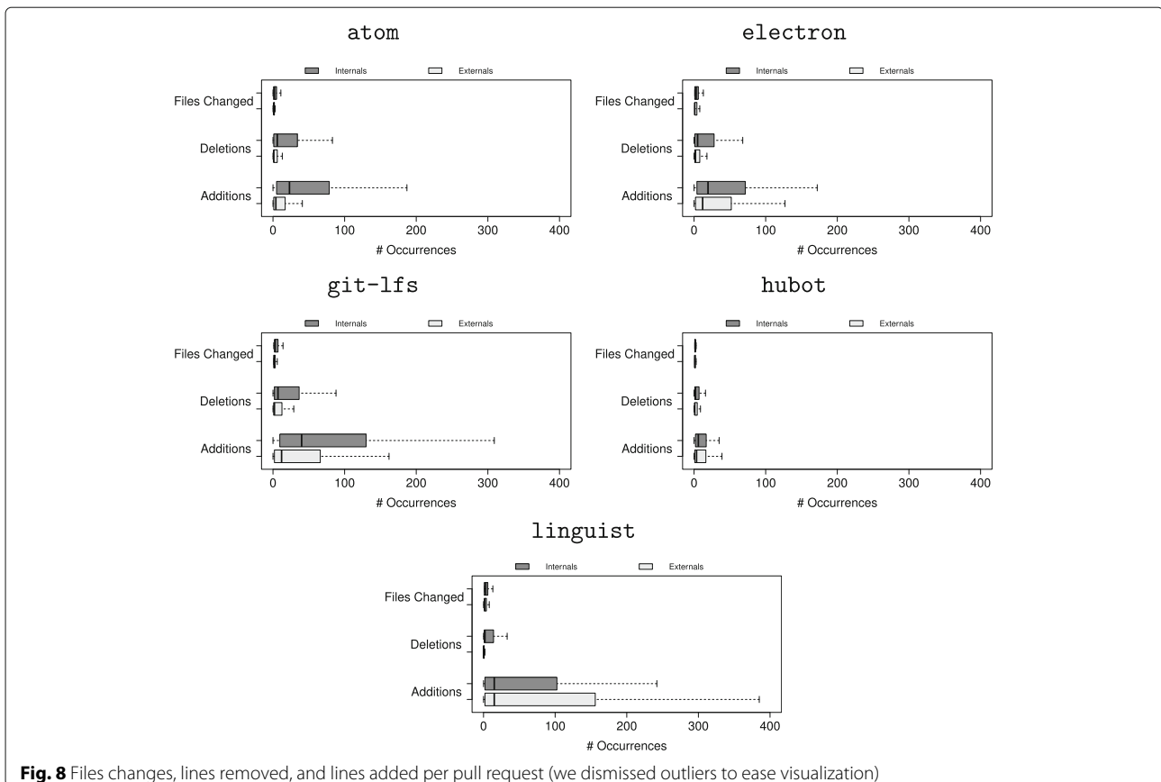
Fig. 8 Files changes, lines removed, and lines added per pull request (we dismissed outliers to ease visualization)
