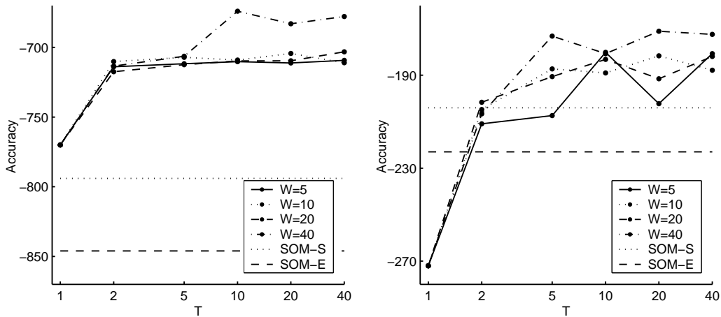
Fig. 6. SOM accuracy for Landsat (left) and Phoneme (right) data as a function of the computational complexity. The effect of the speedup parameter W is not altogether clear, but in general the larger W work better. On the Landsat data the SOM-L results are always better than the comparison methods (SOM-S and SOM-E), but on the Phoneme data the least accurate approximations are not accurate enough.
