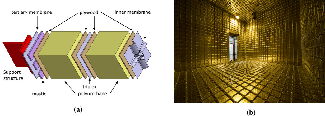
Figure 4. Left: the GTT inner vessel layers. Right: view of the inside of the cryostat ProtoDUNE-SP just after the finalisation of the primary membrane installation. The gold hue visible in the picture is an artifact of the lighting used during the installation, to protect the PDS.
