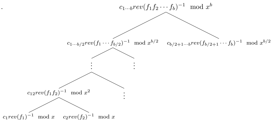
Figure 2: Diagram of the reciprocal tree, where f_i = (Z - x_i) , rev(\cdot) and c_i are as mentioned above.
