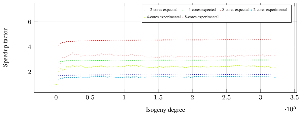
Figure 5: Speedup factors of timings of the joint cost KPS-Parallel + xISOG-Parallel + 2xEVAL-Parallel over \mathbb{F}_{p_{test}} for each odd prime degree \ell \mid (p_{test} + 1) . Experimental timings correspond to an average of 100 runs, whereas the expected savings are obtained from the estimated number of field multiplications from (5) and (6).
