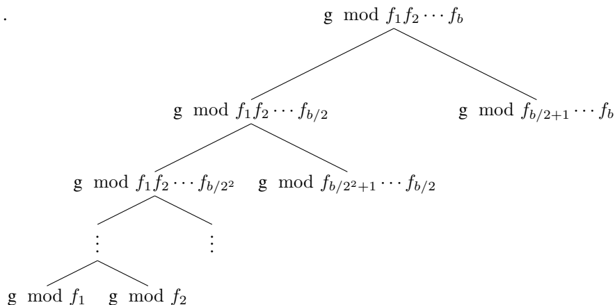
Figure 3: Diagram of the residue tree for computing Res_Z(f(Z), g(Z)) .
