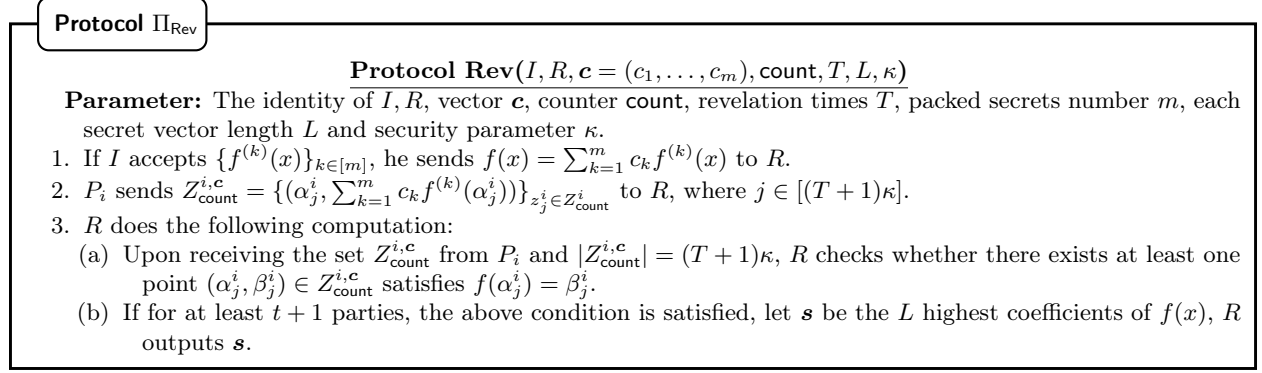
Figure 7: The protocol of the \Pi_{\text{Rev}}
