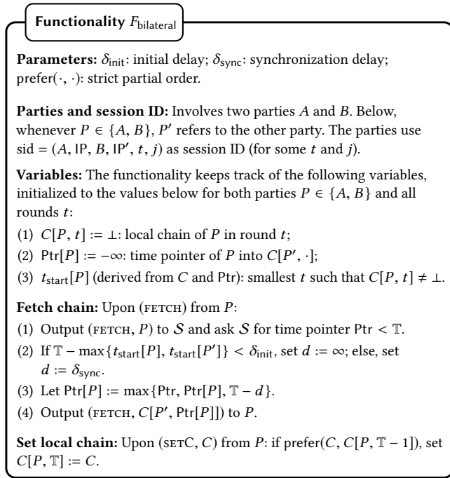
Figure 3: Bilateral chain-sync functionality F_{\text{bilateral}} .
