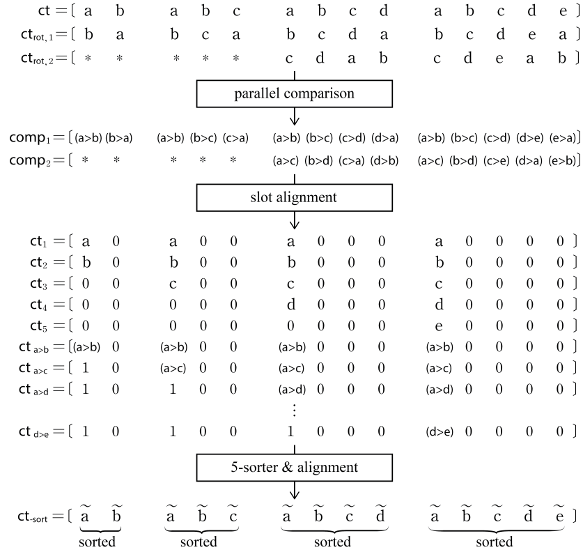
Fig. 4: Illustration of proposed parallel algorithm for the stage with slope 1 in 5-way sorting network. Assuming that all 2- to 5-sorters are run simultaneously, this figure shows the values of each slot in each parallel algorithm step.
