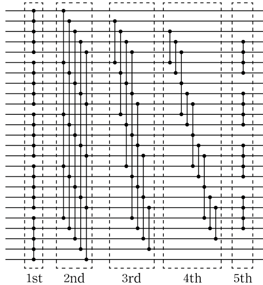
Fig. 3: 5-way sorting network for 5^2 numbers. Each line represents a k -sorter and the multiple dots on each line represent input numbers.
