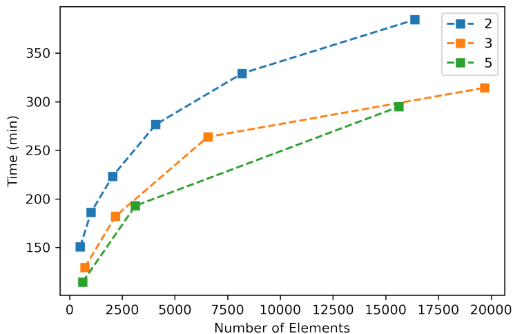
Fig. 6: The illustration of Time and data size from Table 1 with the number of slots s = 2^{15} . Recall that the number of stage for sorting n elements using k -sorting network is O(k \cdot \log_k^2 n) .
